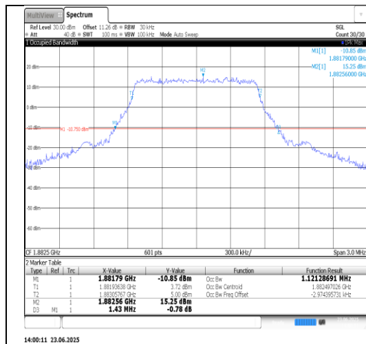
Band25-3MHz-16QAM-26365-15RB#0-PASS
