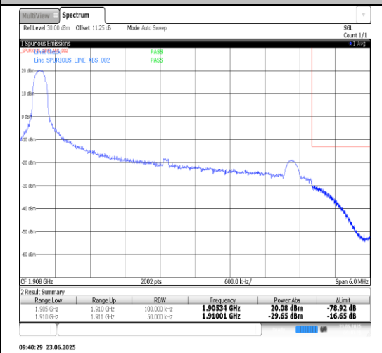
Band2-5MHz-QPSK-19175-25RB#0-PASS
