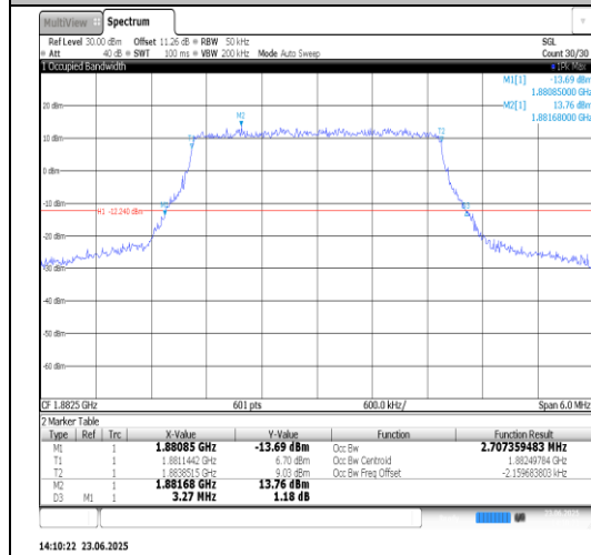
Band25-5MHz-16QAM-26365-25RB#0-PASS
