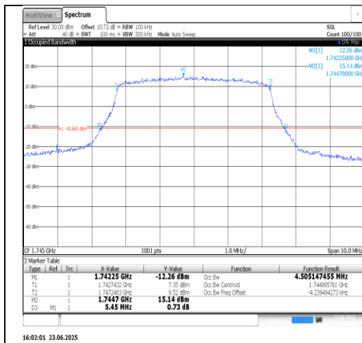
Band66-10MHz-QPSK-132322-50RB#0-PASS
