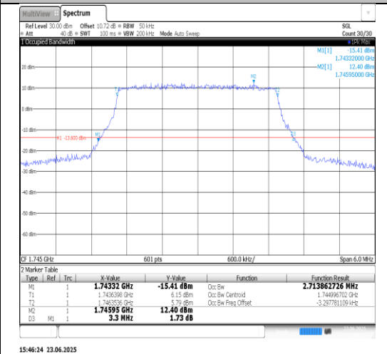
Band66-5MHz-16QAM-132322-25RB#0-PASS
