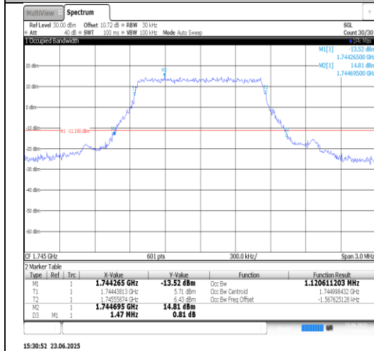
Band66-3MHz-QPSK-132322-15RB#0-PASS
