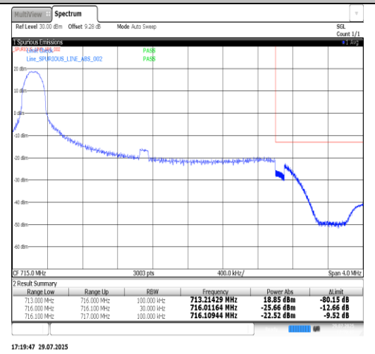
Band12-3MHz-QPSK-23165-1RB#14-PASS_Final1
