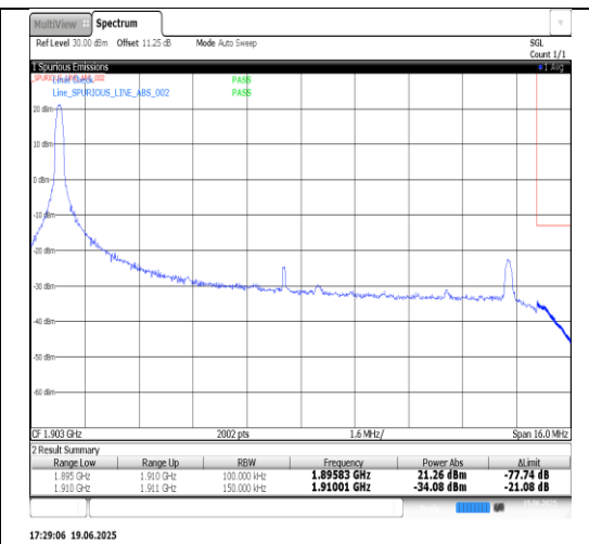
Band2-15MHz-QPSK-19125-75RB#0-PASS
