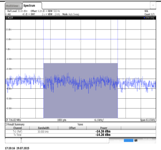
Band12-3MHz-16QAM-23025-1RB#0-PASS
