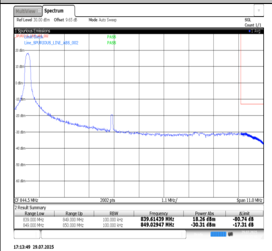
Band5-10MHz-16QAM-20600-1RB#49-PASS_Final1
