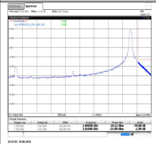
Band2-15MHz-QPSK-18675-1RB#74-PASS
