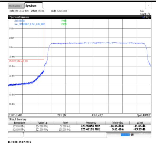
Band5-3MHz-16QAM-20635-1RB#14-PASS
