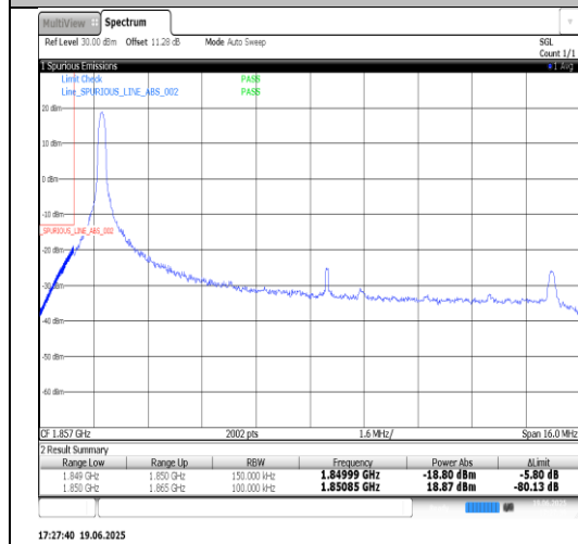
Band2-15MHz-QPSK-18675-75RB#0-PASS
