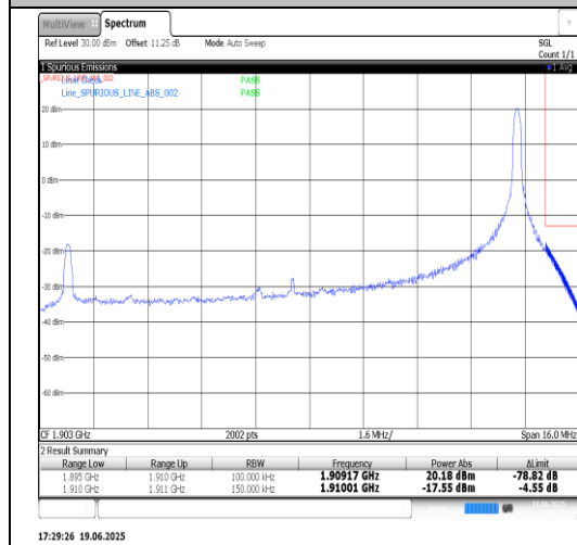
Band2-15MHz-16QAM-18675-1RB#0-PASS
