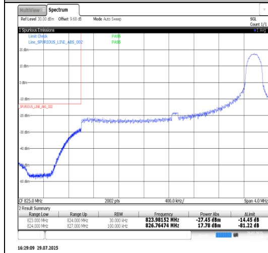
Band5-3MHz-16QAM-20635-1RB#0-PASS
