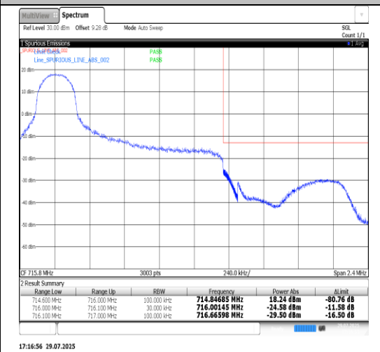
Band12-1.4MHz-16QAM-23173-6RB#0-PASS
