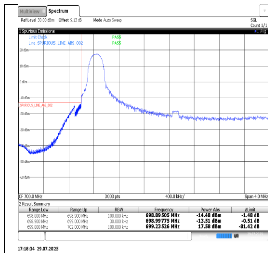
Band12-3MHz-QPSK-23025-15RB#0-PASS
