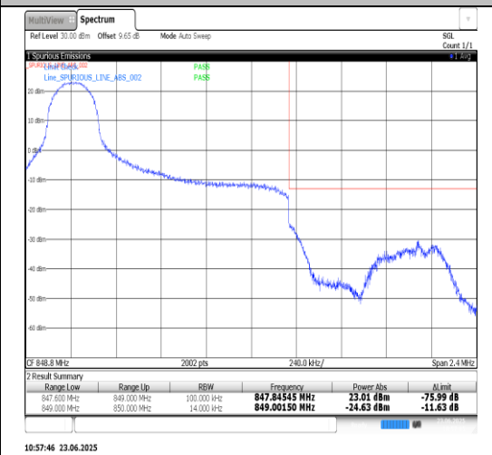
Band5-1.4MHz-QPSK-20643-6RB#0-PASS
