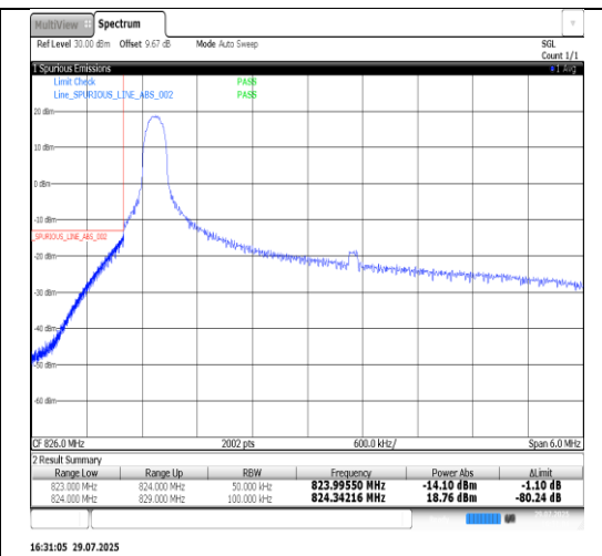
Band5-5MHz-QPSK-20425-25RB#0-PASS
