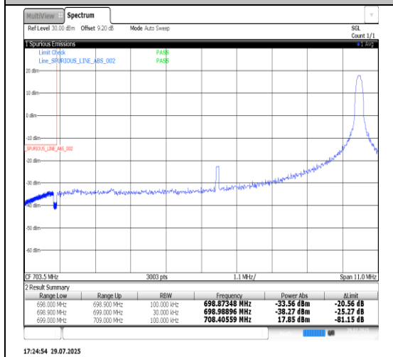
Band12-10MHz-16QAM-23130-1RB#49-PASS
