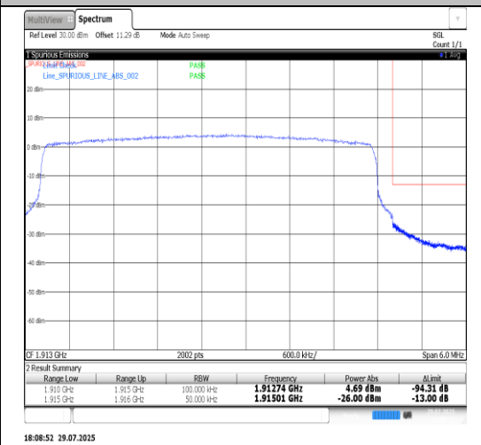
Band25-5MHz-16QAM-26065-1RB#24-PASS
