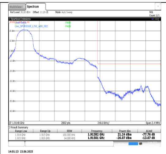
Band25-1.4MHz-QPSK-26683-6RB#0-PASS
