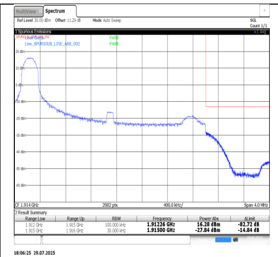
Band25-3MHz-16QAM-26675-15RB#0-PASS
