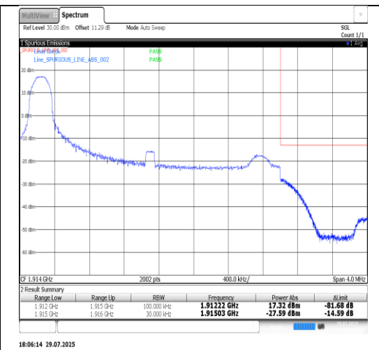
Band25-3MHz-QPSK-26675-15RB#0-PASS
