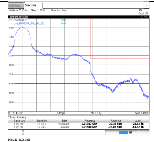
Band25-1.4MHz-16QAM-26683-6RB#0-PASS
