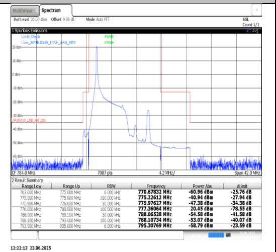
Band13-5MHz-QPSK-23205-25RB#0-PASS
