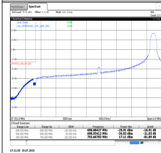
Band12-5MHz-16QAM-23155-1RB#0-PASS
