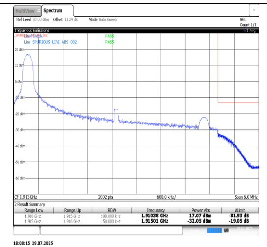
Band25-5MHz-QPSK-26665-25RB#0-PASS
