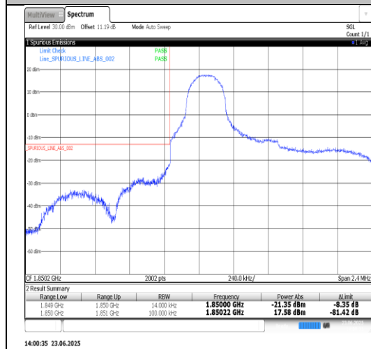
Band25-1.4MHz-16QAM-26047-6RB#0-PASS
