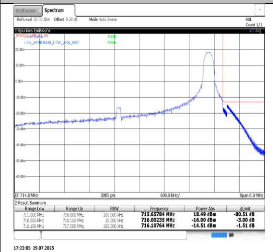
Band12-10MHz-QPSK-23060-1RB#0-PASS
