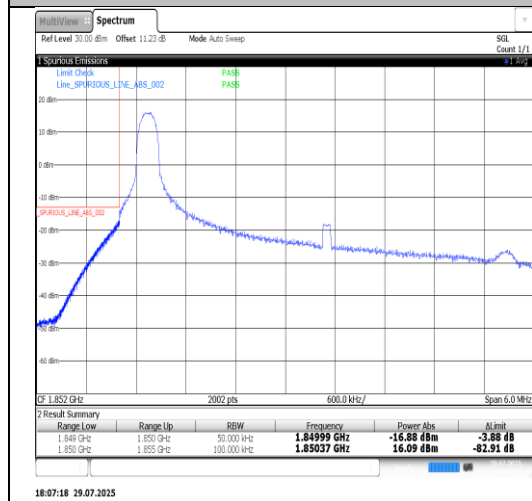
Band25-5MHz-QPSK-26065-25RB#0-PASS
