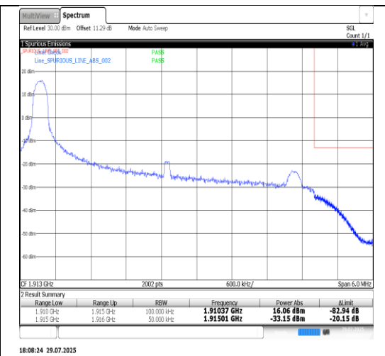
Band25-5MHz-16QAM-26665-25RB#0-PASS
