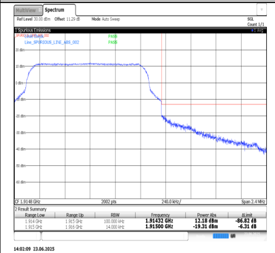
Band25-3MHz-QPSK-26055-1RB#14-PASS
