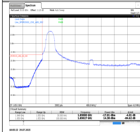
Band25-3MHz-16QAM-26055-15RB#0-PASS
