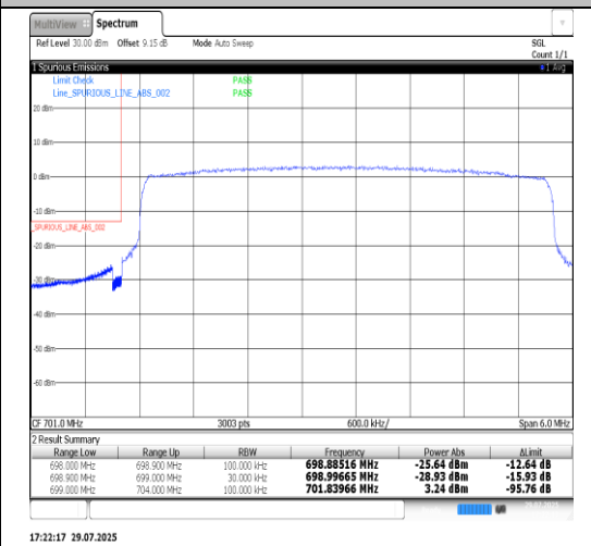
Band12-5MHz-16QAM-23155-1RB#24-PASS
