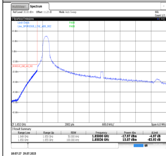
Band25-5MHz-16QAM-26065-25RB#0-PASS
