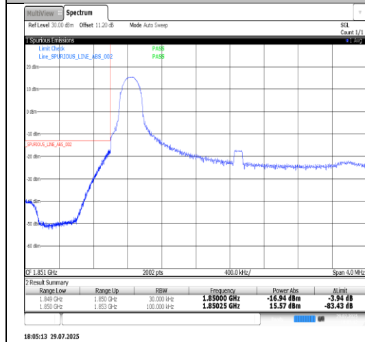
Band25-3MHz-QPSK-26055-15RB#0-PASS
