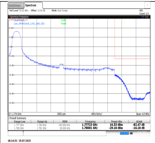
Band66-3MHz-QPSK-132657-15RB#0-PASS
