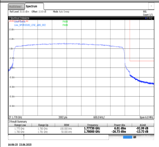
Band66-10MHz-QPSK-132022-1RB#49-PASS
