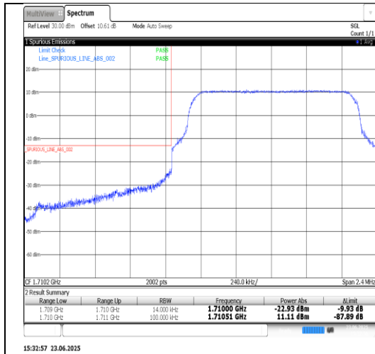
Band66-1.4MHz-QPSK-132665-1RB#5-PASS
