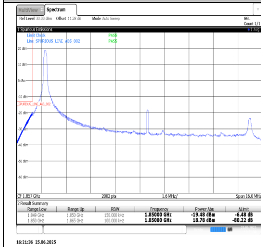
Band25-15MHz-QPSK-26115-75RB#0-PASS
