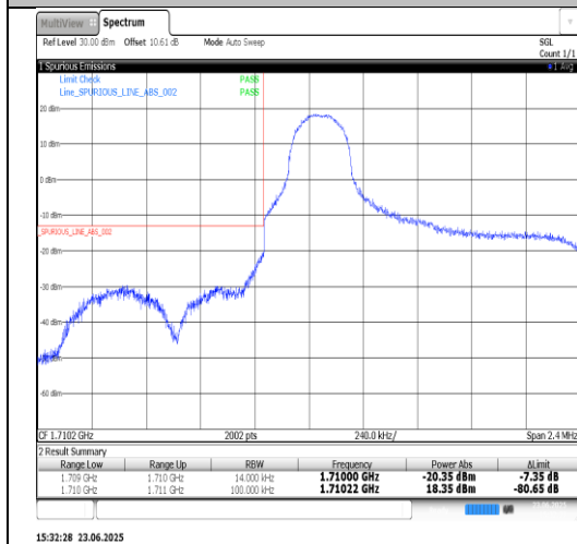
Band66-1.4MHz-16QAM-131979-6RB#0-PASS
