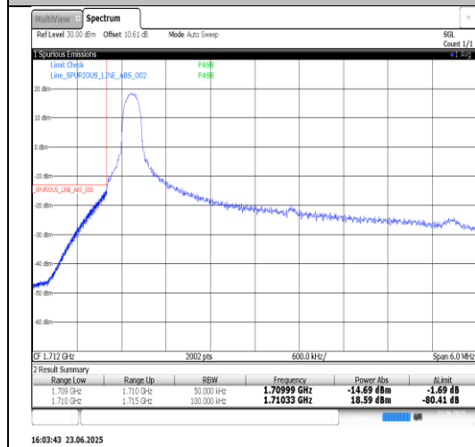
Band66-5MHz-16QAM-131997-25RB#0-PASS
