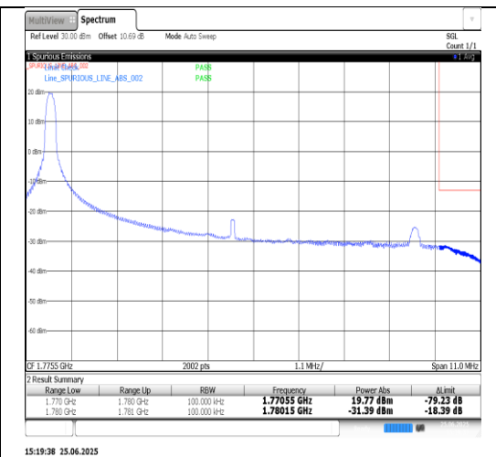
Band66-10MHz-QPSK-132622-50RB#0-PASS
