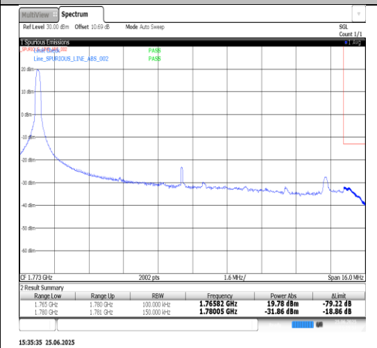
Band66-15MHz-QPSK-132597-75RB#0-PASS
