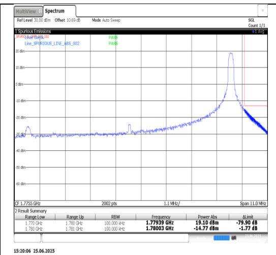
Band66-15MHz-QPSK-132047-1RB#74-PASS
