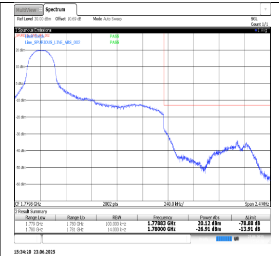
Band66-1.4MHz-QPSK-132665-6RB#0-PASS
