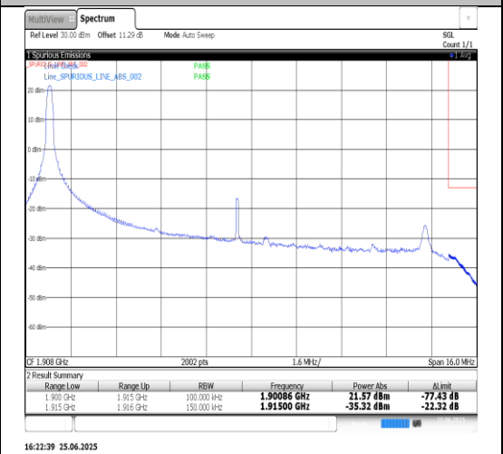
Band25-15MHz-QPSK-26615-75RB#0-PASS
