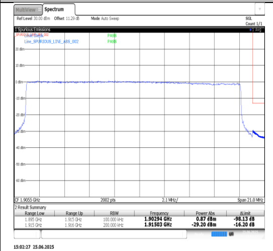
Band25-20MHz-16QAM-26140-1RB#99-PASS
