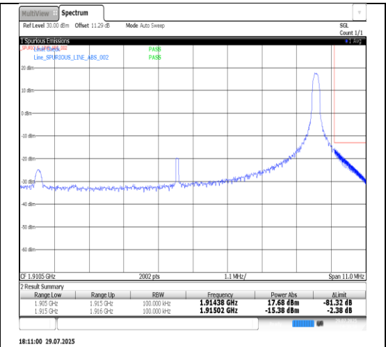
Band25-15MHz-QPSK-26115-1RB#74-PASS
