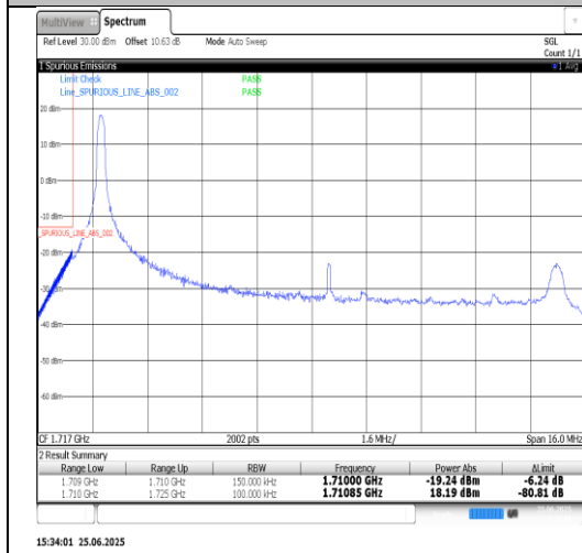
Band66-15MHz-16QAM-132597-1RB#0-PASS
