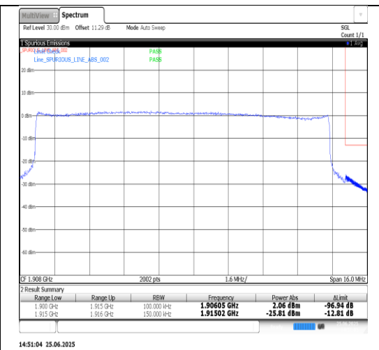
Band25-15MHz-16QAM-26115-1RB#74-PASS
