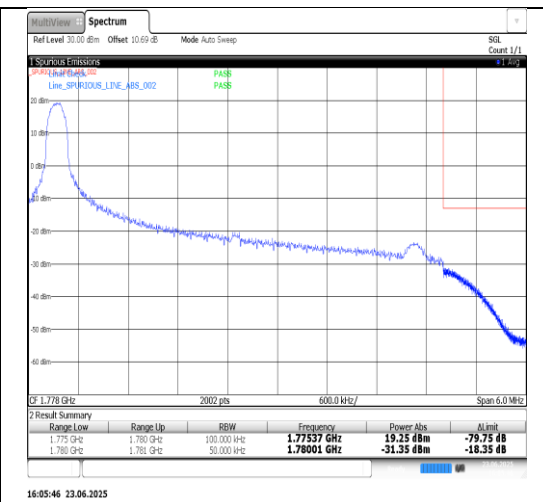
Band66-5MHz-16QAM-132647-25RB#0-PASS
