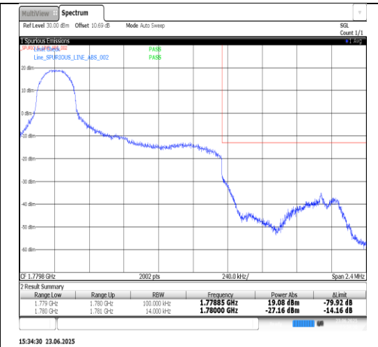
Band66-1.4MHz-16QAM-132665-6RB#0- PASS
