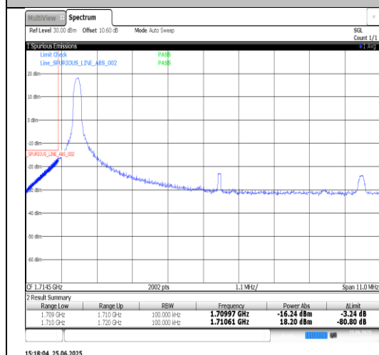
Band66-10MHz-16QAM-132622-1RB#0-PASS
