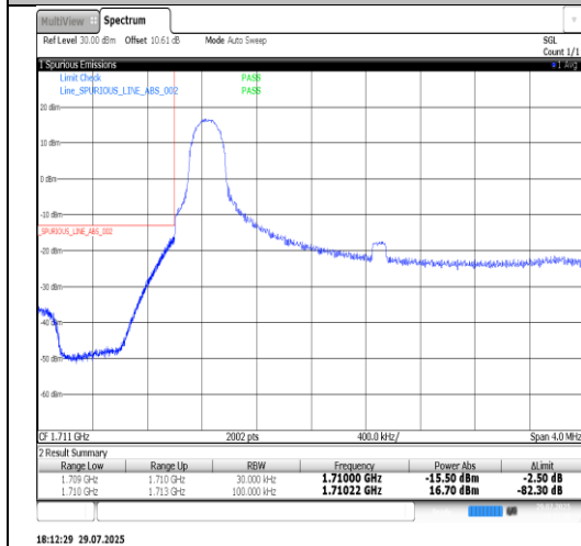
Band66-3MHz-QPSK-131987-15RB#0-PASS
