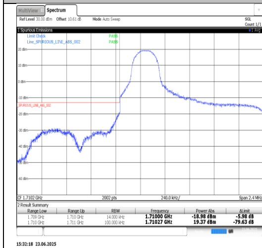
Band66-1.4MHz-QPSK-131979-6RB#0-PASS
