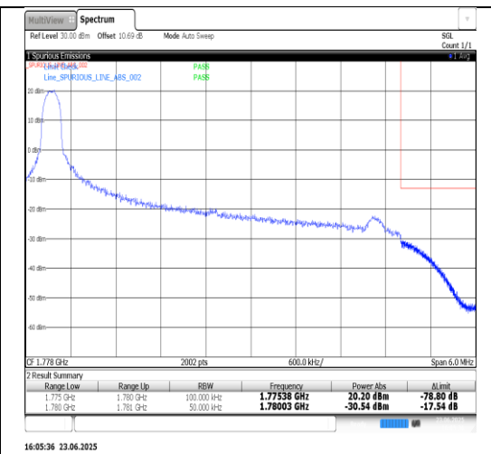
Band66-5MHz-QPSK-132647-25RB#0-PASS
