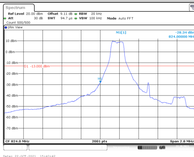
Band26-1.4MHz-QPSK-26797-6-0-Low--35.59-PASS
