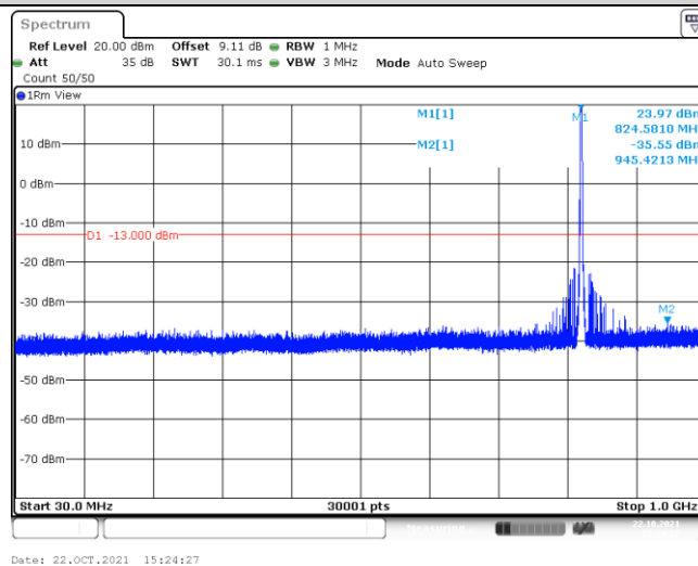
Band26-1.4MHz-16QAM-26797-6-0-Low-1000-5000--40.63-PASS
