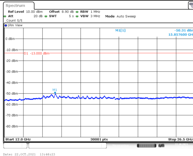
Band85-5MHz-QPSK-134027-6-0-Low-30-1000--35.61-PASS
