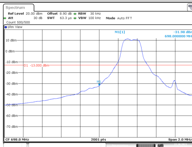
Band85-5MHz-QPSK-134027-1-0-Low--31.98-PASS
