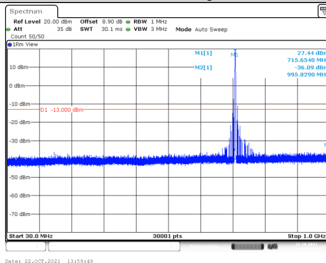
Band85-5MHz-QPSK-134157-1-5-High-1000-5000--40.95-PASS
