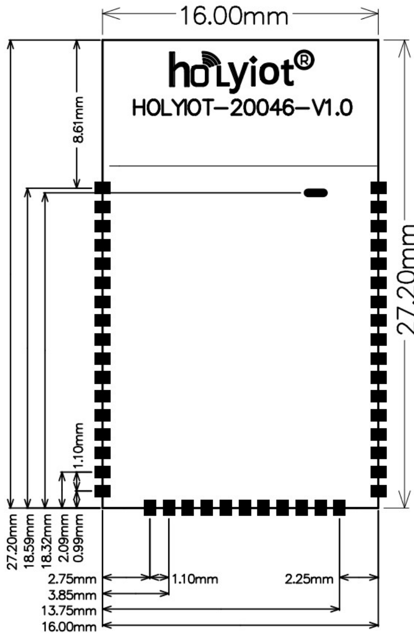
TOP VIEW
