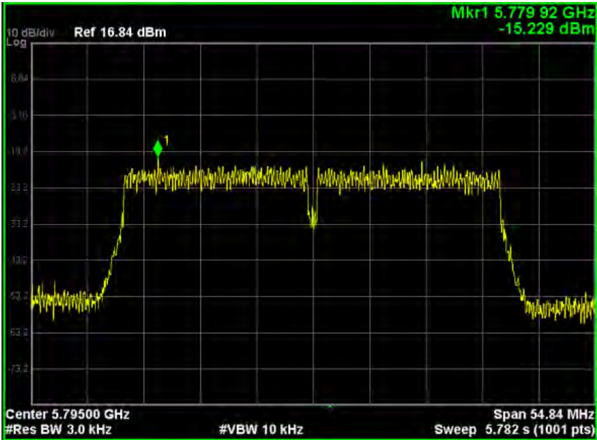
802.11ac40 channel 159
