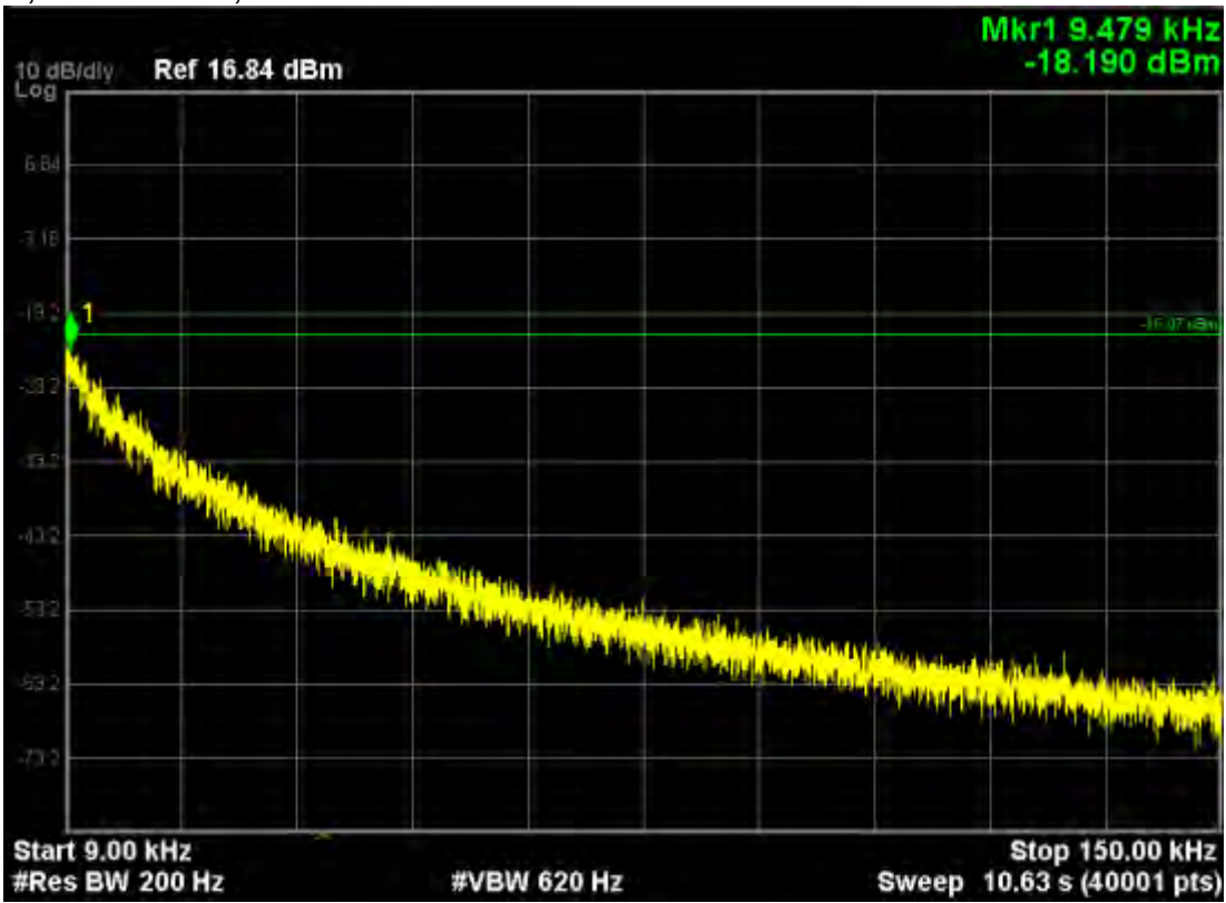
802.11b, traffic mode; Channel6
