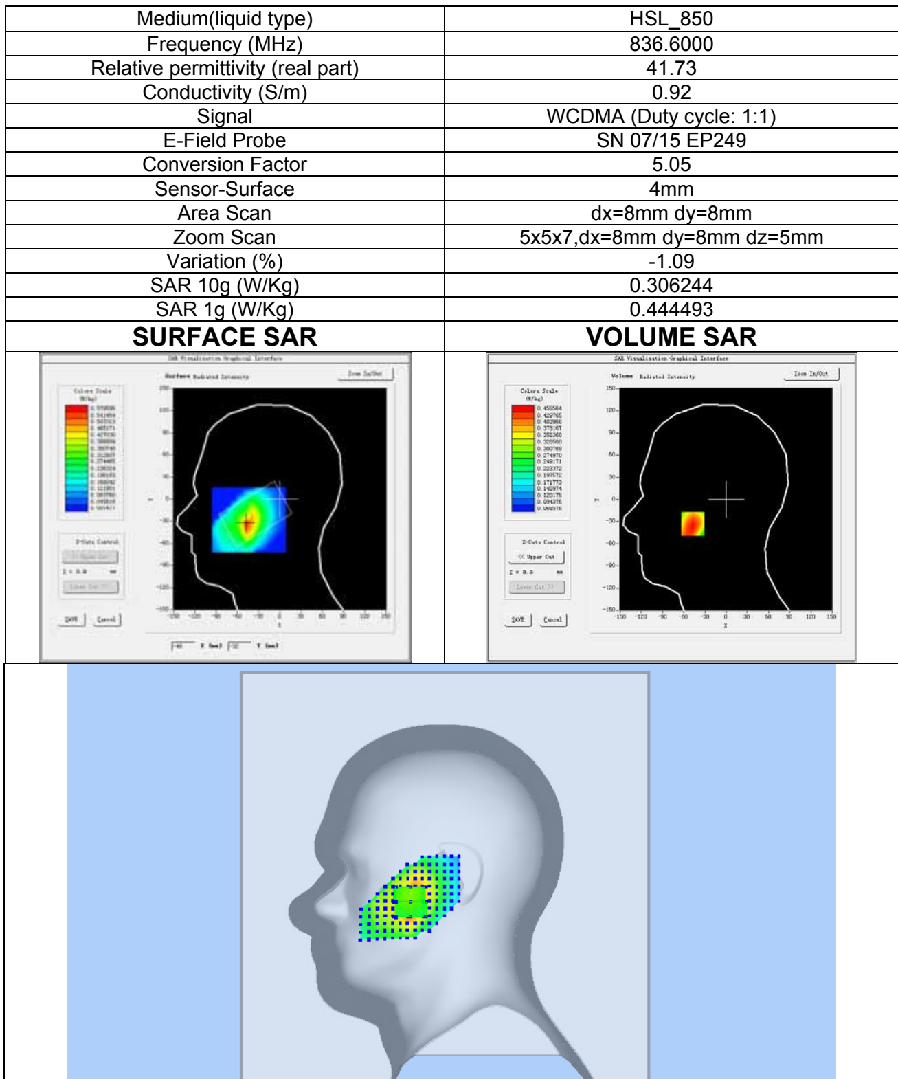
Plot 7: WCDMA BAND V, Middle channel (Right Head Cheek) Product Description: Mobile Phone Test Date: Mar 19,2017
