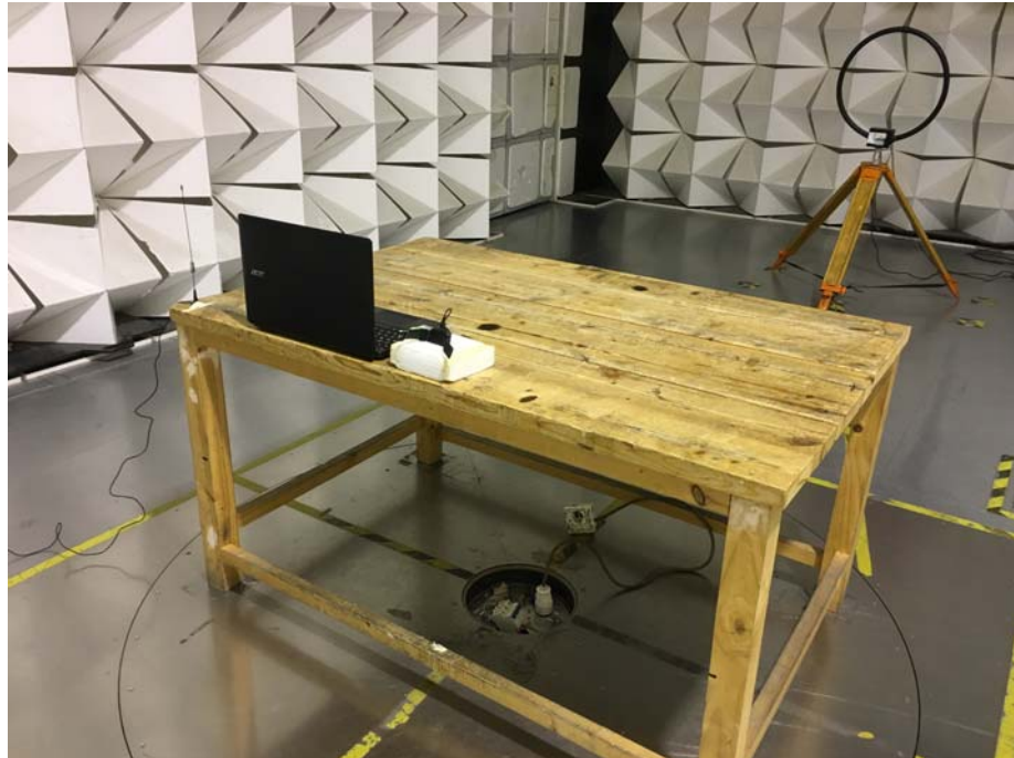
Below 30MHz
