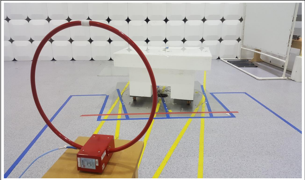
Radiated Emission 9 kHz ~ 30 MHz
