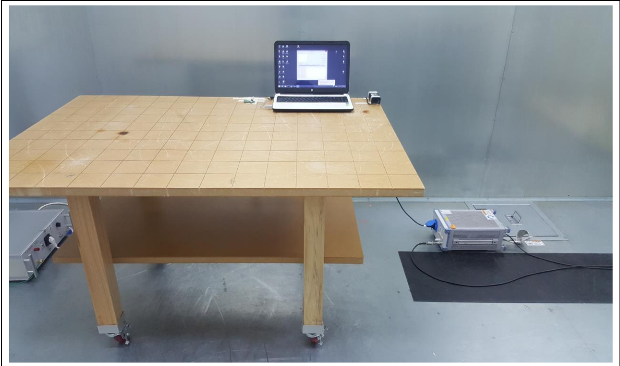
Conducted Emission FRONT
