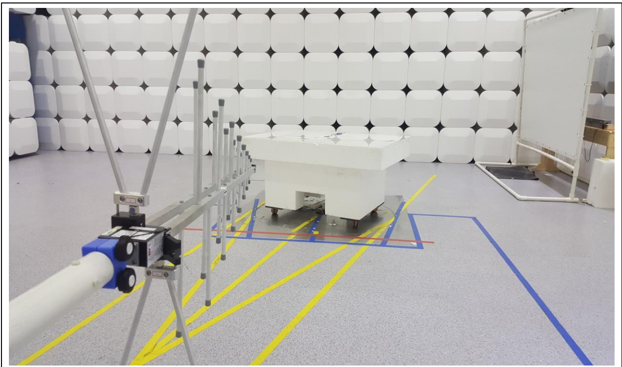
Radiated Emission 30 MHz ~ 1 GHz
