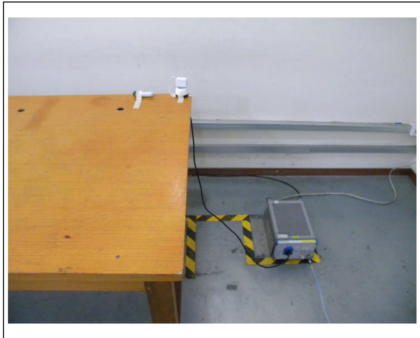
Photo of AC Power line emission Test
