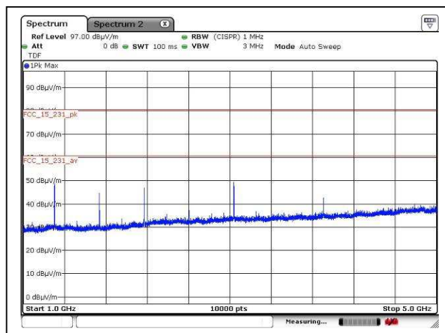
Lower channel, 1GHz – 5GHz, Vertical
