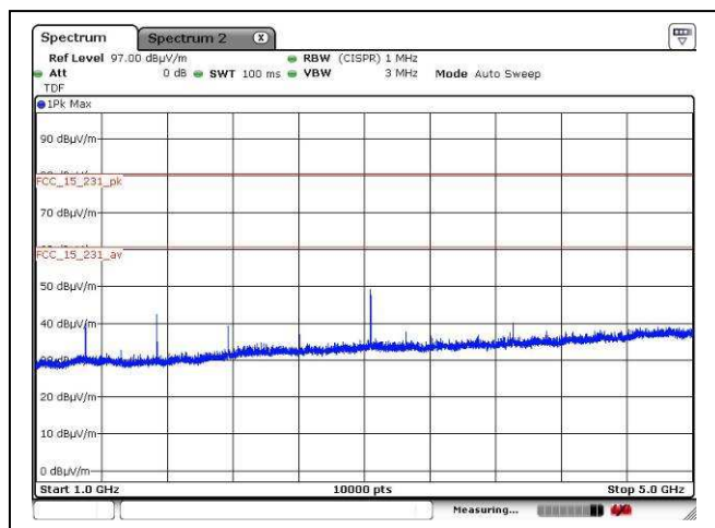
Lower channel, 1GHz – 5GHz, Horizontal
