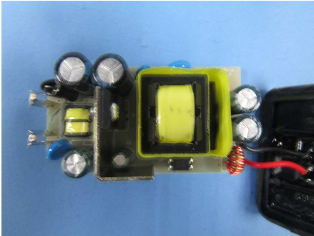
Power supply PCB view
