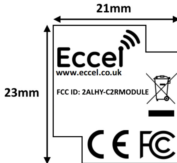
Figure 1- Identification label (laser engraver) appearance and dimensions:
