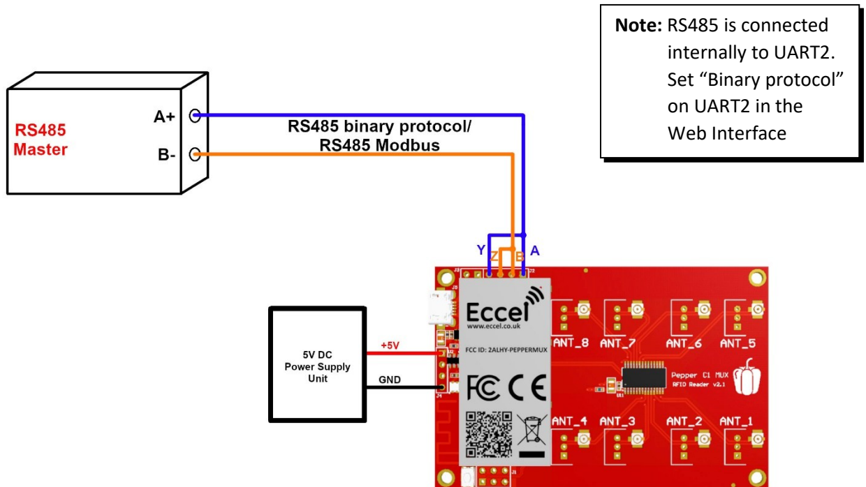
Figure 3-7. Pepper C1 FCC MUX RS485 - half duplex connection schematic
