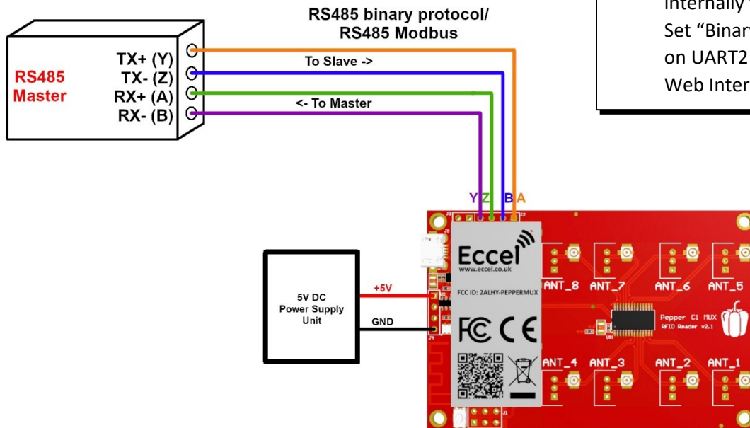
Figure 3-5. Pepper C1 FCC RS485 - full duplex connection example
