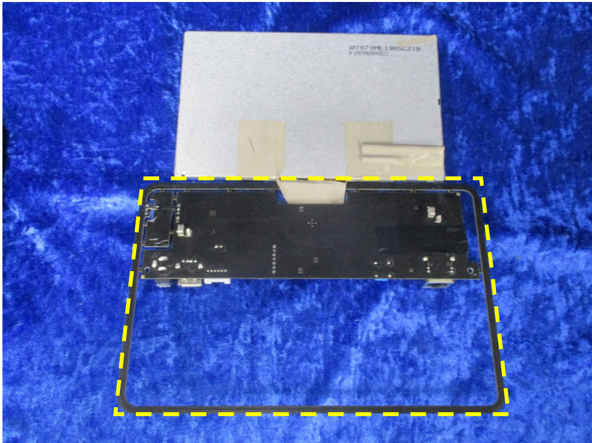
PCB etched coil antenna (highlighted)
