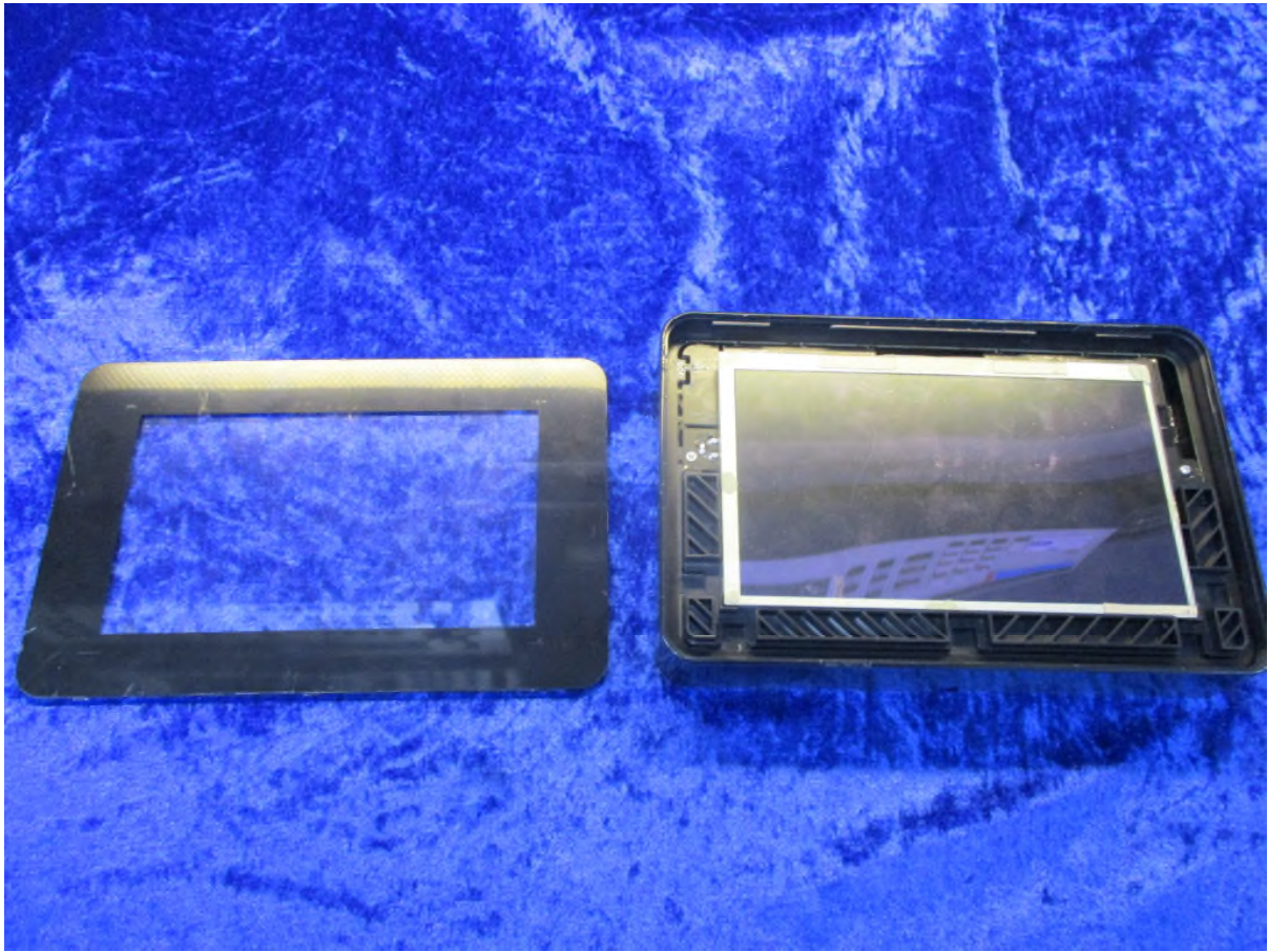
Pcb and display in chassis – protective screen removed
