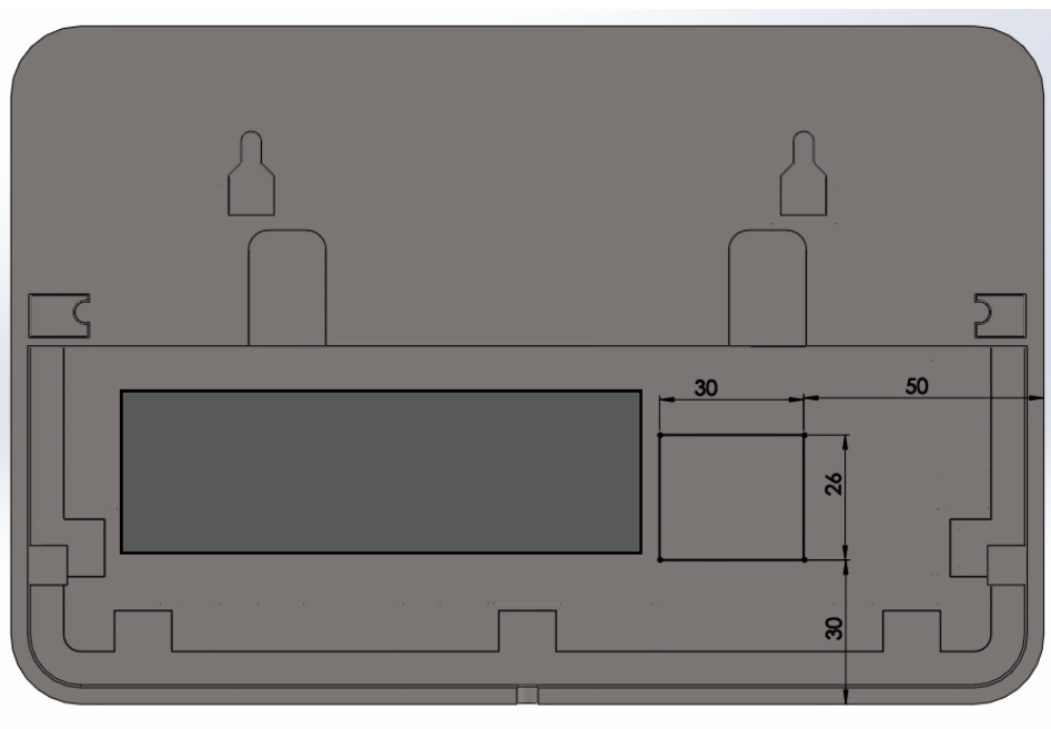
Figure 3- Back face of Action Cam User device showing positioning of labels.
