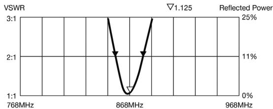
The Linx ANT-868-CW-HWR-SMA antenna is used for 865...869 MHz (ZMEERAZBERRY7_ANT)
