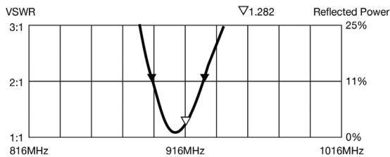
The Linx ANT-916-CW-HWR-SMA antenna is used for 908...917, 919...921 MHz (ZMEURAZBERRY7_ANT)
