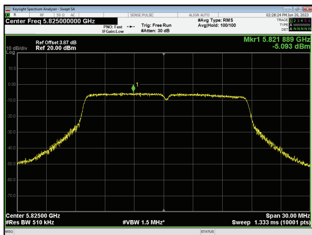
(802.11a20) PSD plot on channel 165
