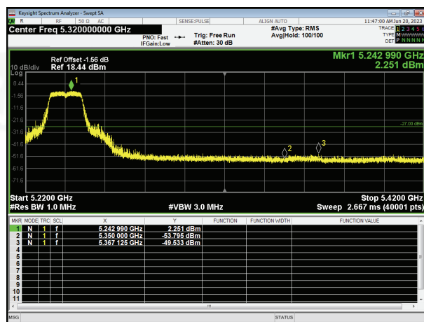
Band Edge ac20 5240MHz High
