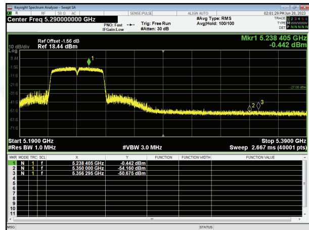
Band Edge n20 5240MHz High
