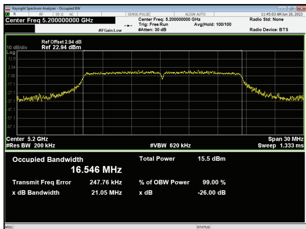
(802.11 a20) 26dB Bandwidth plot on channel 40
