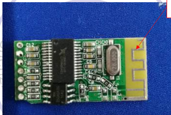
BT Antenna
