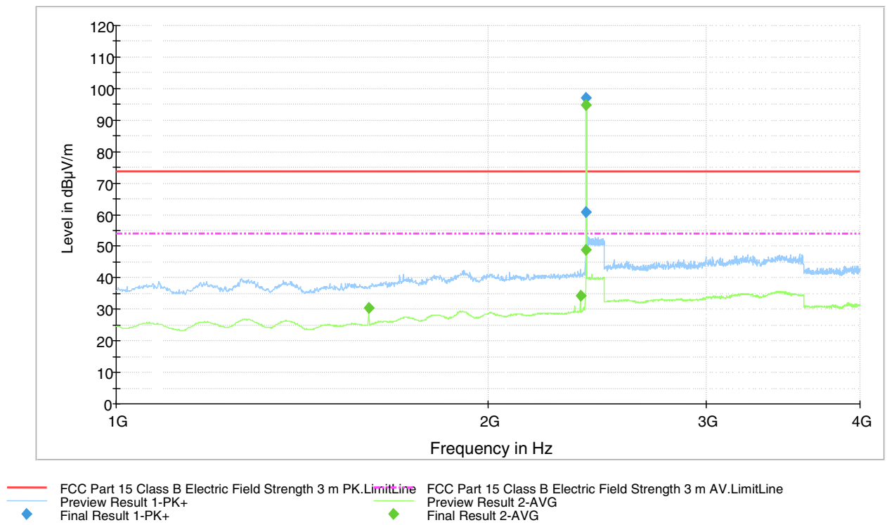
Figure 14. Measured curve with peak- and average detector. 1 Mbps Channel LOW.
