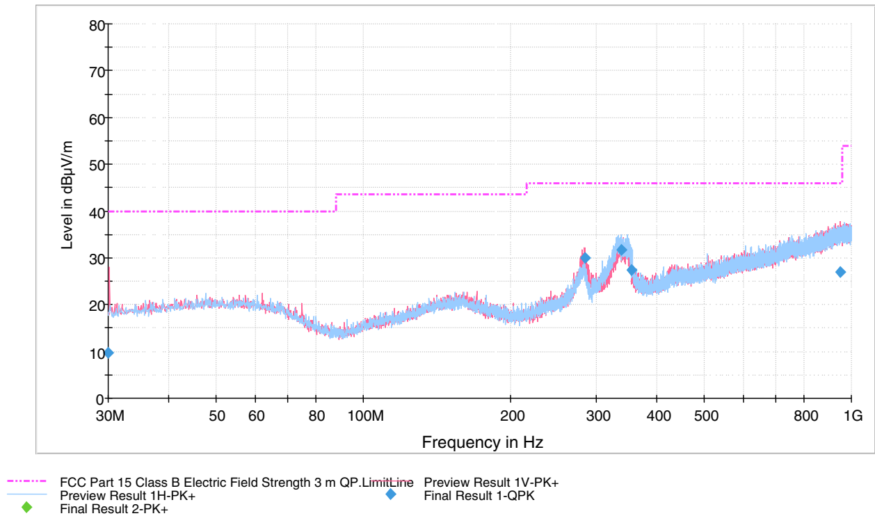
Figure 27. Measured curve with peak-detector. 1 Mbps Channel HIGH.
