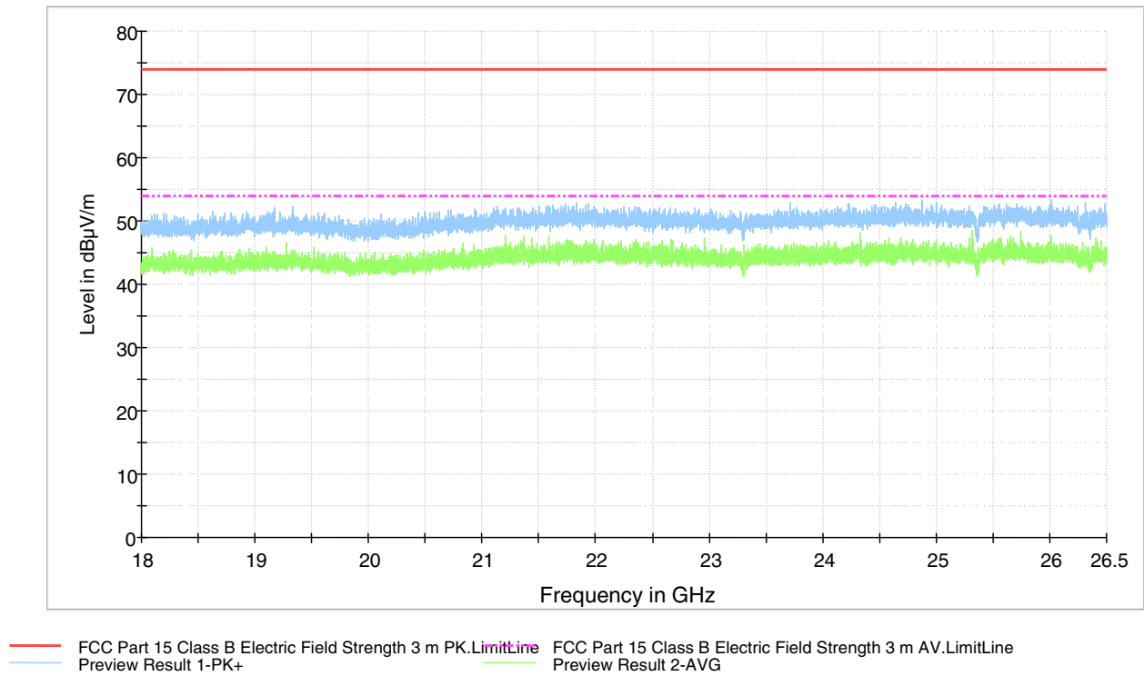
Figure 24. Measured curve with peak- and average detector. 1 Mbps Channel HIGH.
