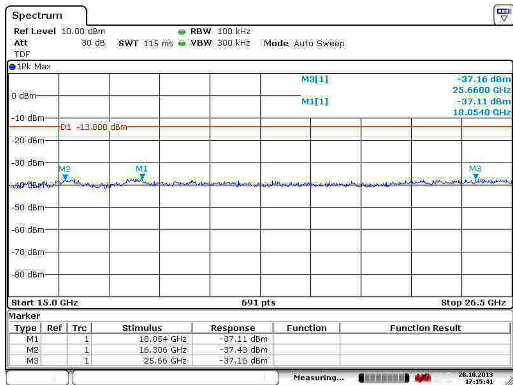
Figure 51. Mid channel conductive emission 15 GHz to 26.5 GHz (1 Mbps).
