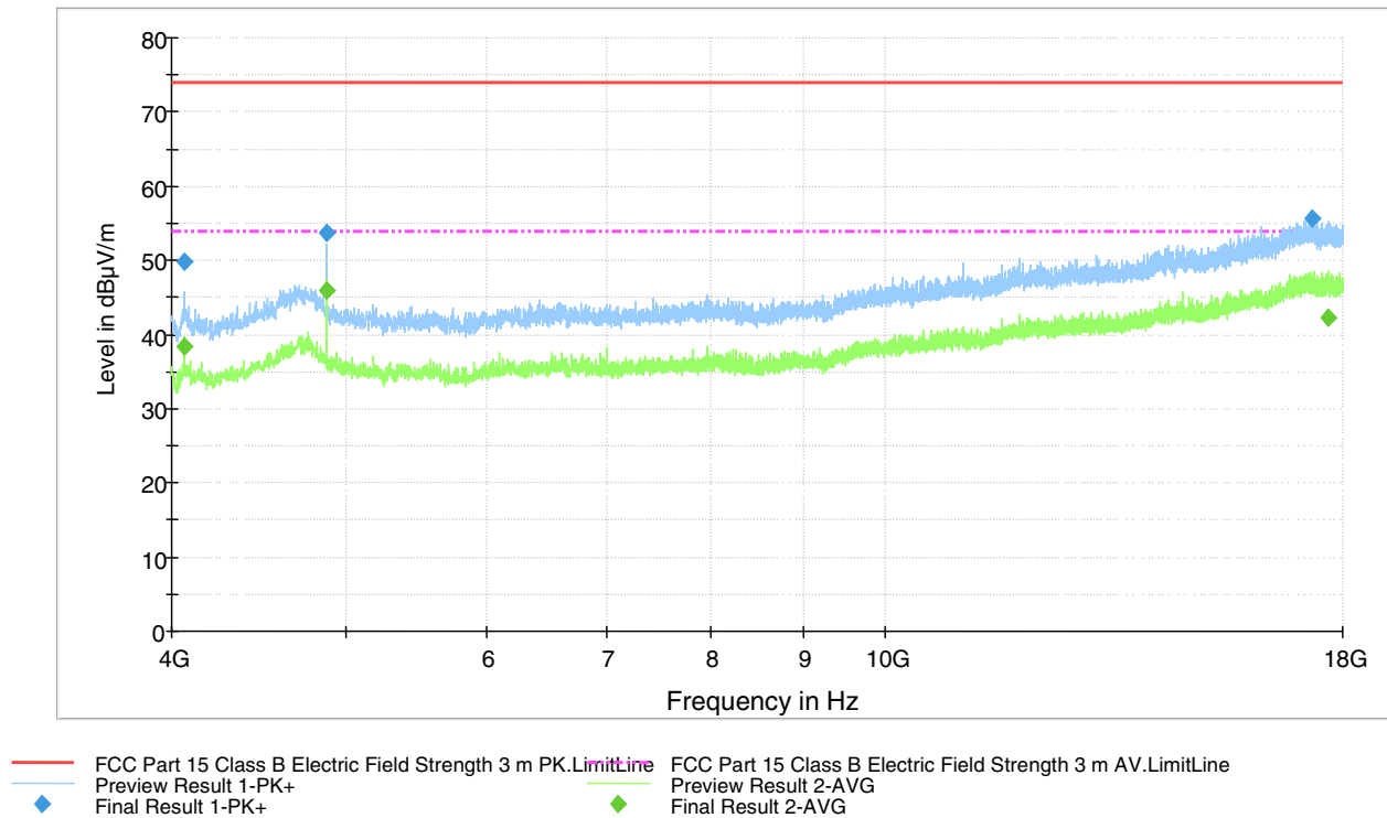
Figure 34. Measured curve with peak- and average detector. 1 Mbps Channel MID.
