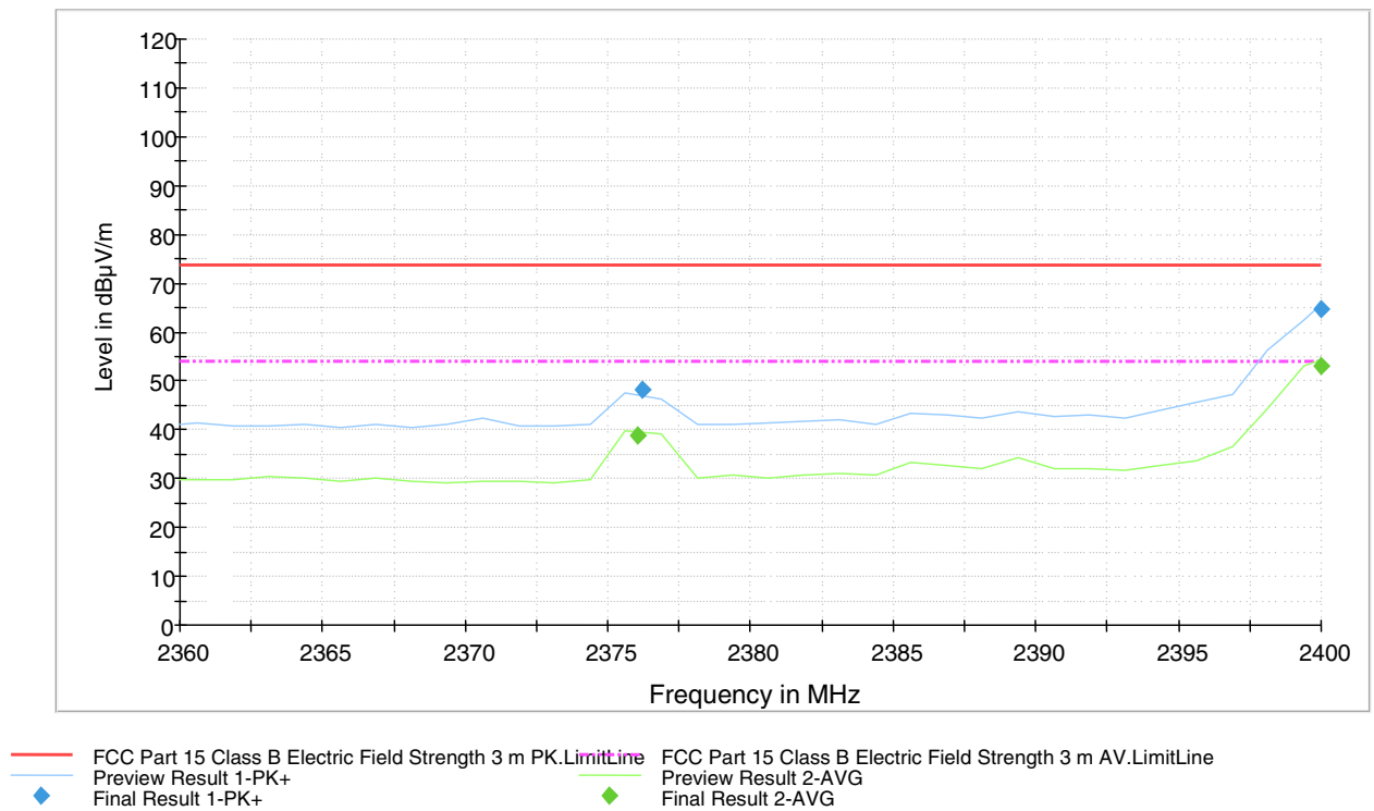
Figure 29. Low channel band edge 1 Mbps.
