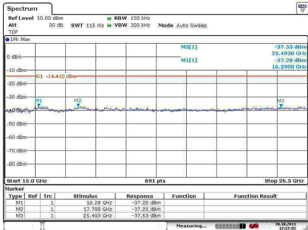
Figure 66. High channel conductive emission 15 GHz to 26.5 GHz (2 Mbps).
