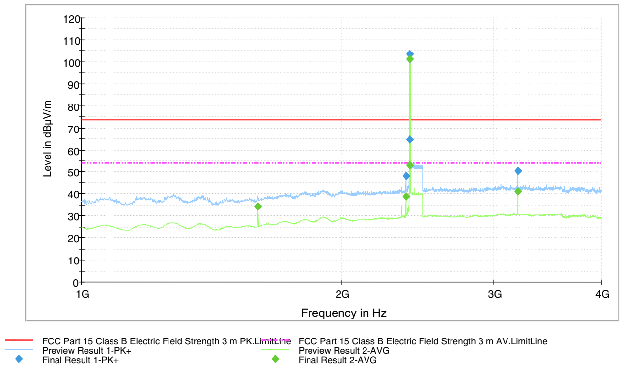
Figure 28. Measured curve with peak- and average detector. 1 Mbps Channel LOW.
