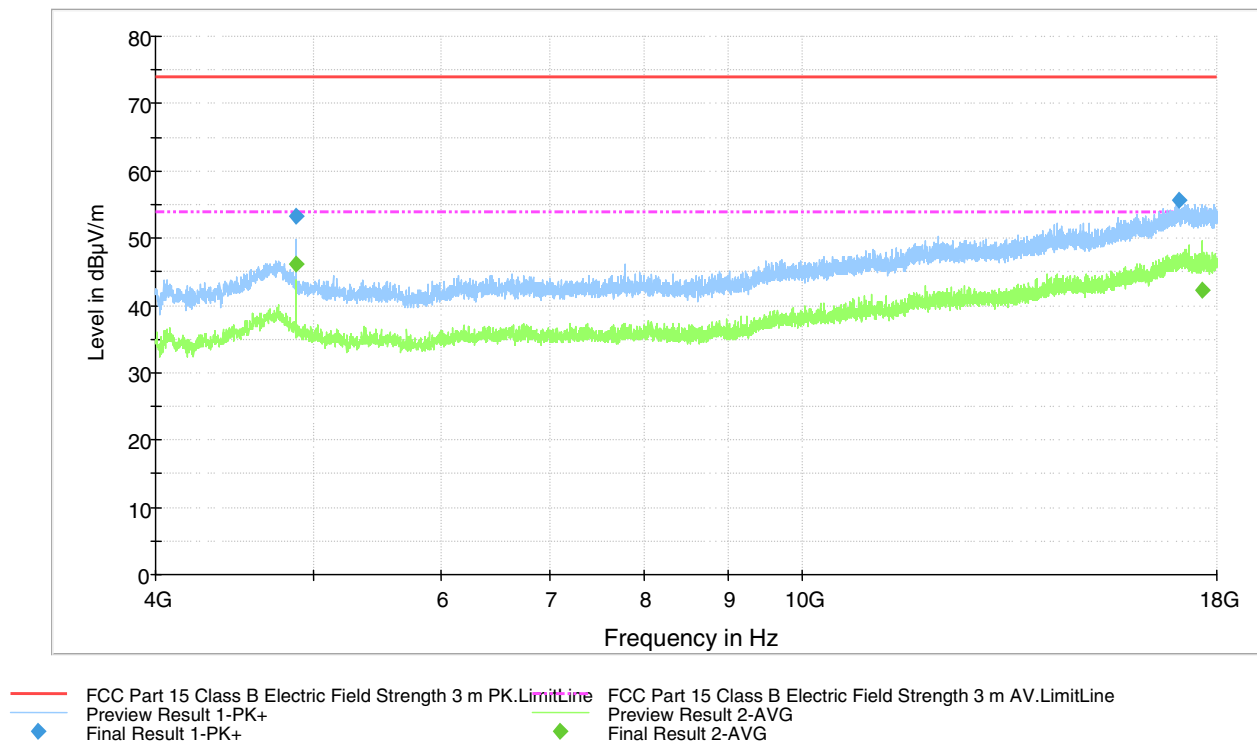
Figure 20. Measured curve with peak- and average detector. 1 Mbps Channel MID.
