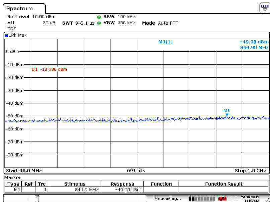
Figure 67. Low channel conductive emission 30 MHz to 1000 MHz (3 Mbps).
