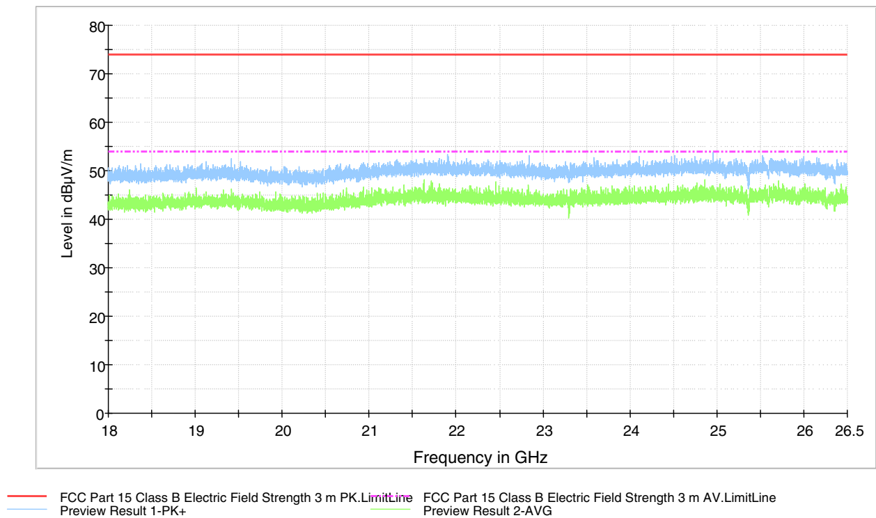
Figure 38. Measured curve with peak- and average detector. 1 Mbps Channel HIGH.
