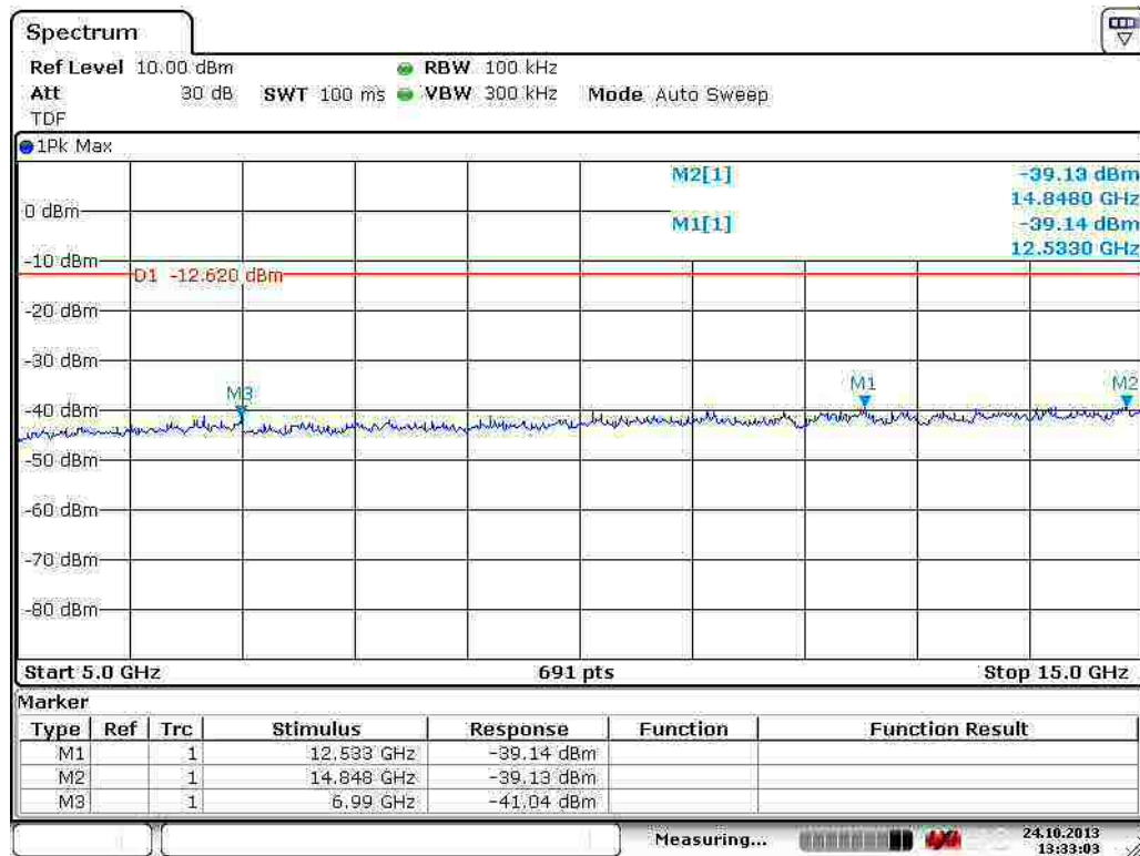
Figure 47. Low channel conductive emission 5 GHz to 15 GHz (1 Mbps).
