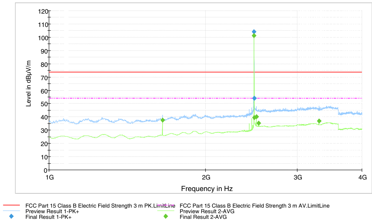
Figure 31. Measured curve with peak- and average detector. 1 Mbps Channel HIGH.
