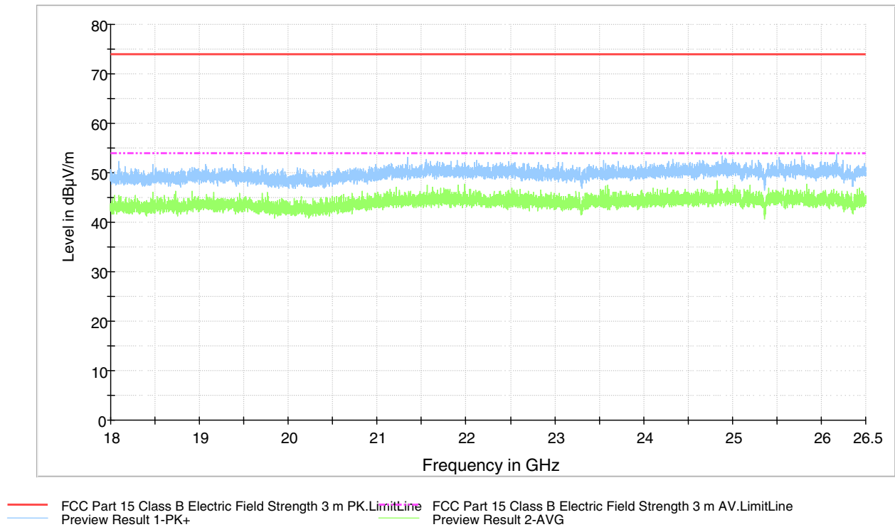
Figure 37. Measured curve with peak- and average detector. 1 Mbps Channel MID.
