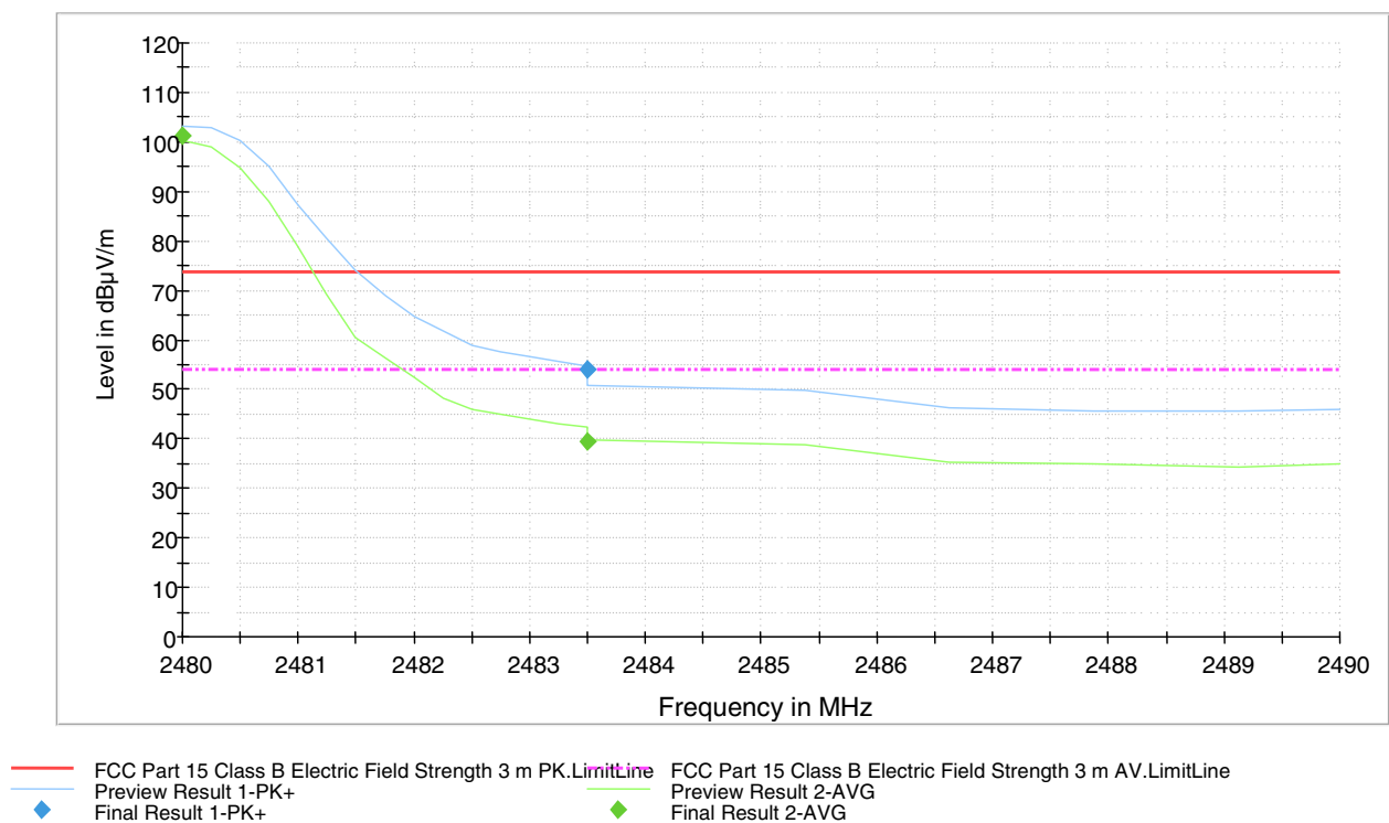
Figure 32. High channel edge 1 Mbps.
