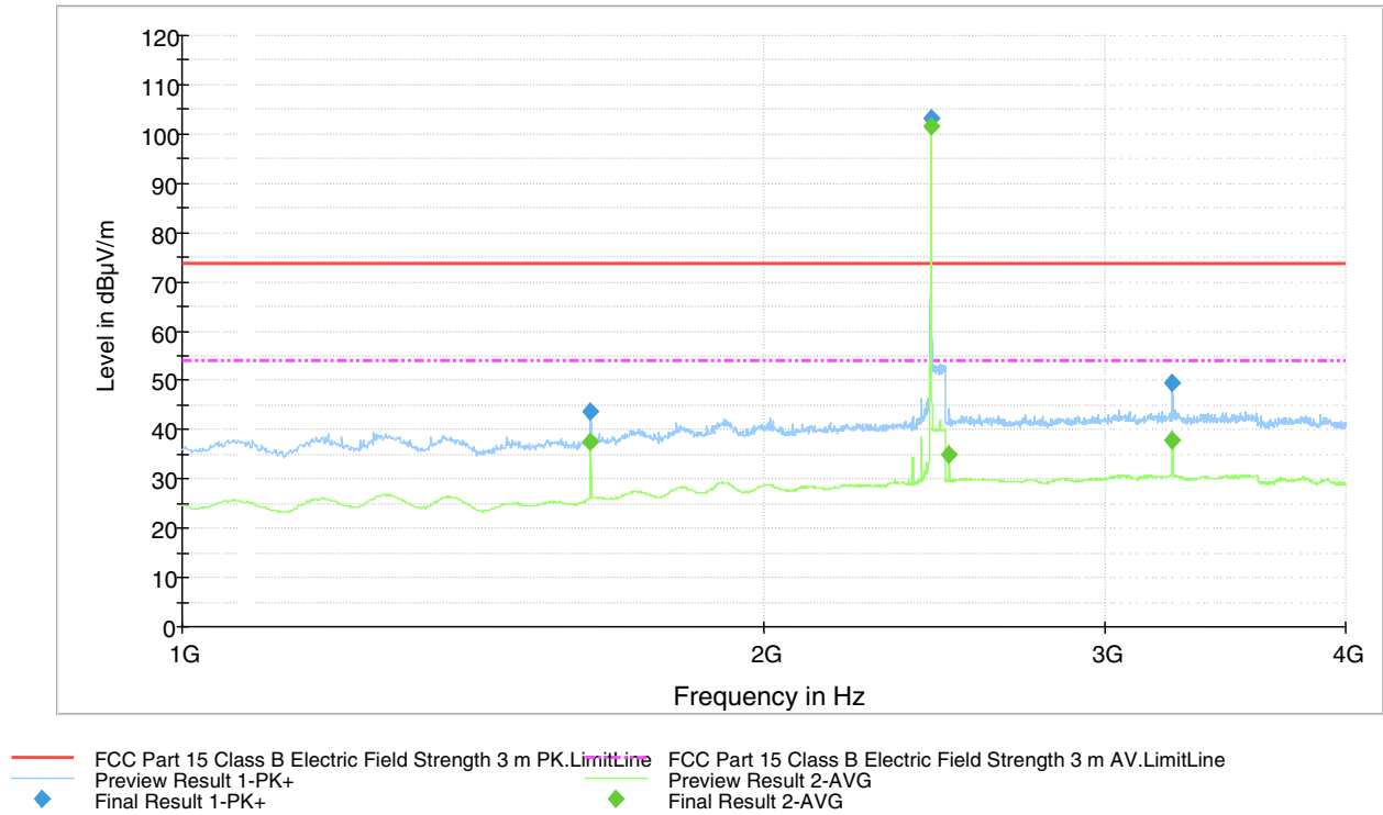
Figure 30. Measured curve with peak- and average detector. 1 Mbps Channel MID.
