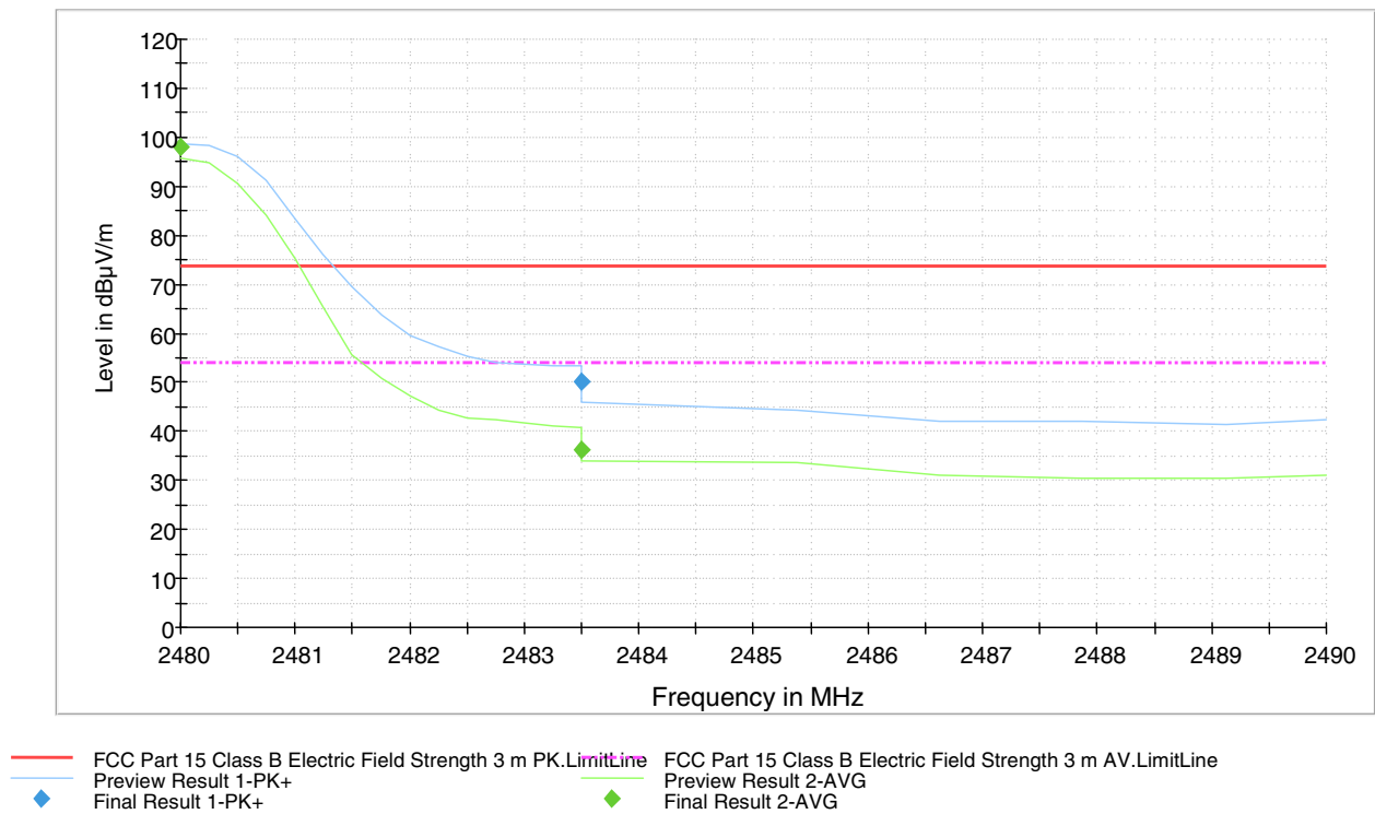
Figure 18. High channel band edge 1 Mbps.
