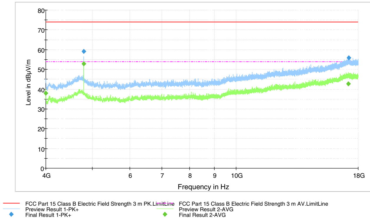
Figure 33. Measured curve with peak- and average detector. 1 Mbps Channel LOW.
