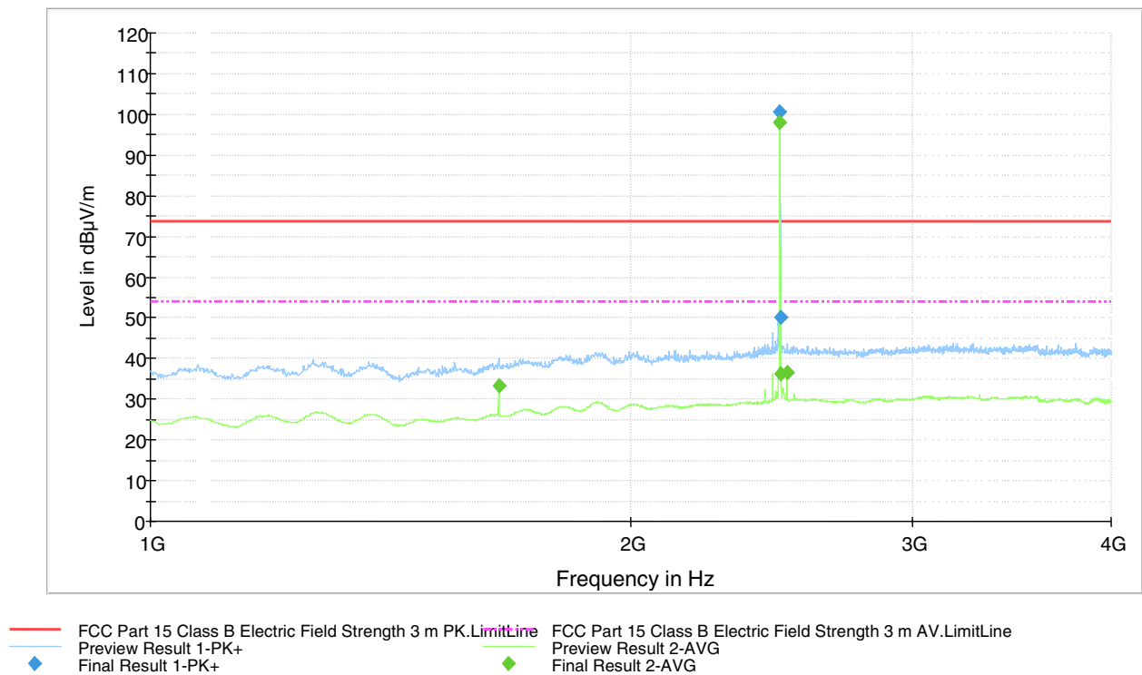
Figure 17. Measured curve with peak- and average detector. 1 Mbps Channel HIGH.
