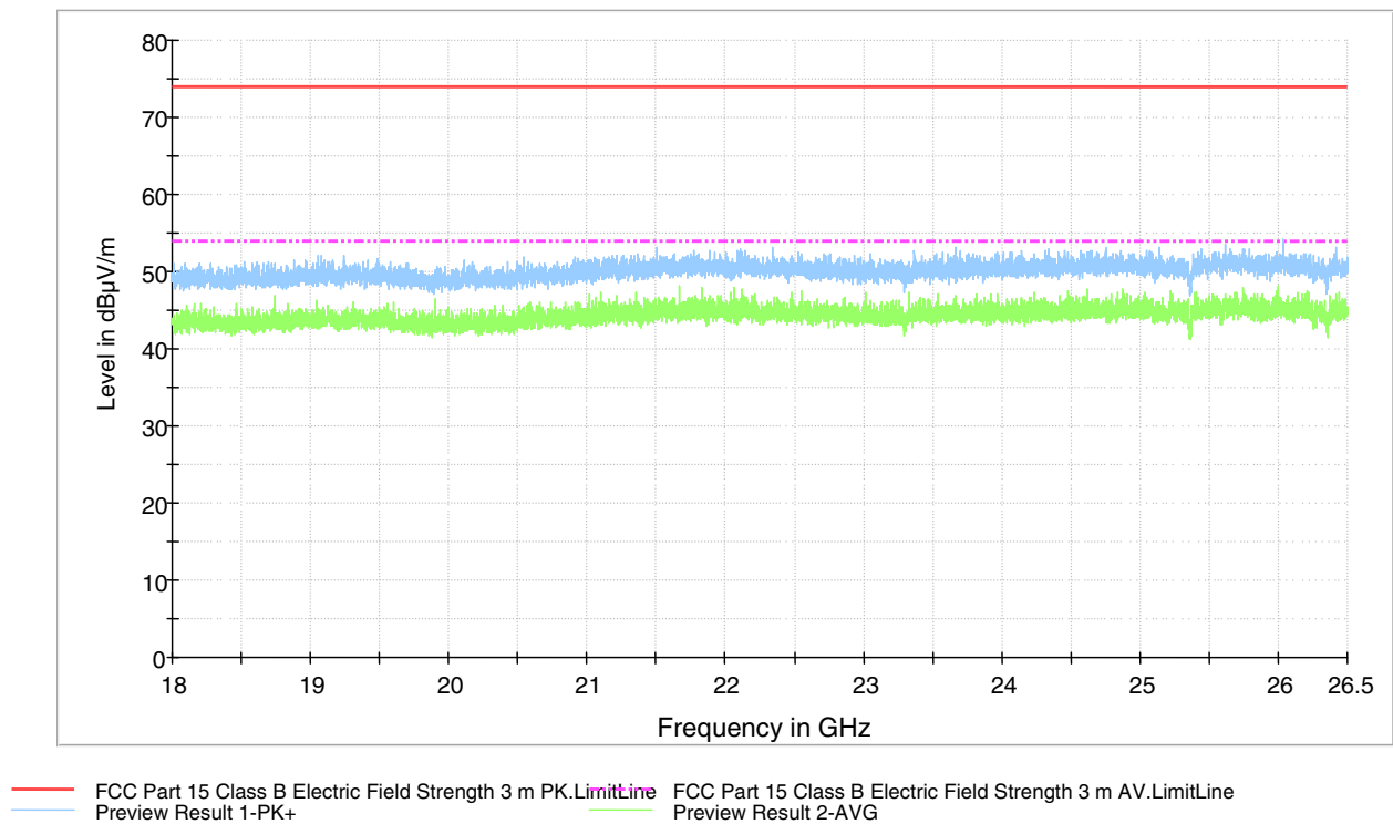
Figure 22. Measured curve with peak- and average detector. 1 Mbps Channel LOW.
