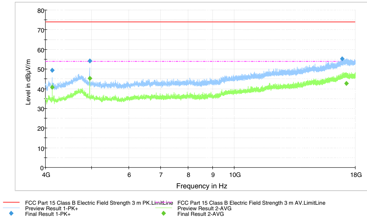
Figure 35. Measured curve with peak- and average detector. 1 Mbps Channel HIGH.
