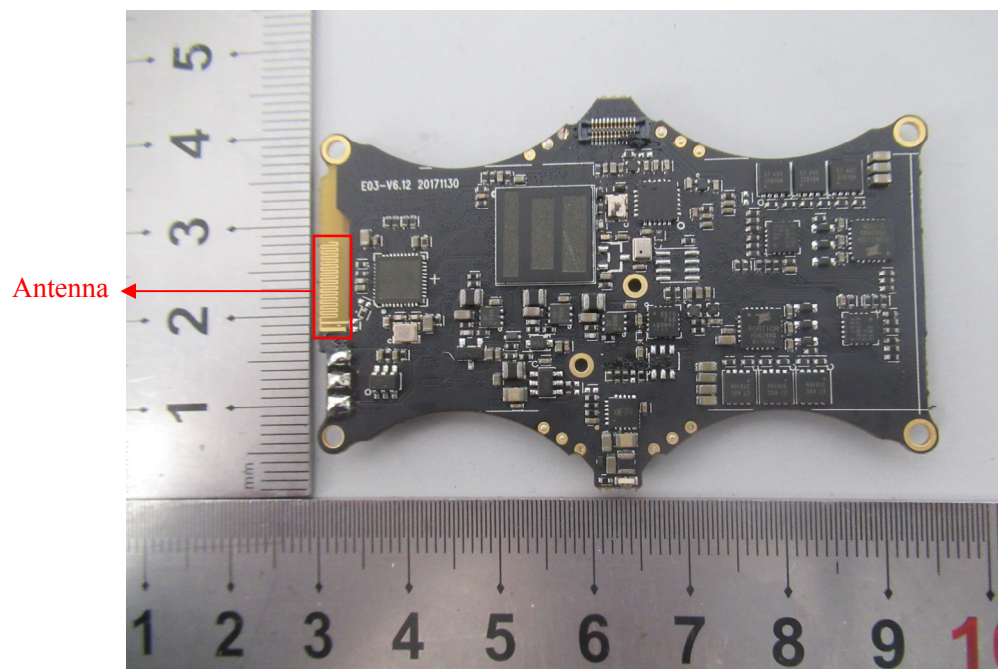
EUT – PCB-2 Top View
