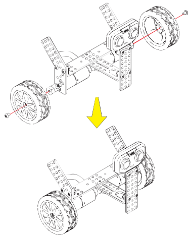
Step 7: install the wheels
