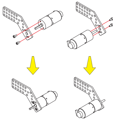
Step 1: install the right and left motor
