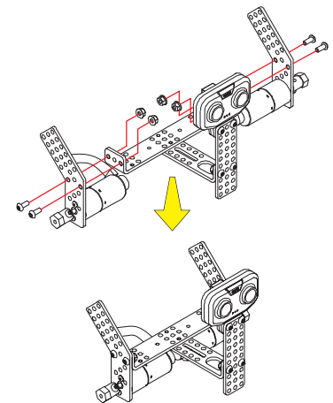
Step 6: install the motor assemblies
