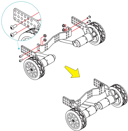
Step 5: attach the wheel assemblies to the front bracket
