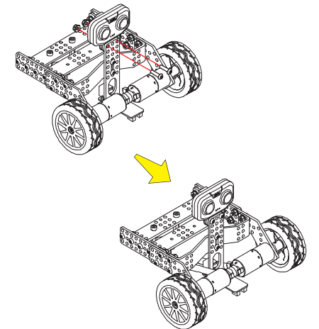
Step 11: install the ultrasonic sensor
