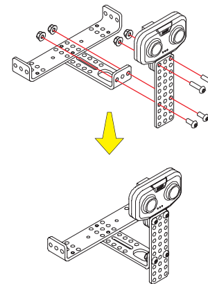
Step 5: install ultrasonic sensor
