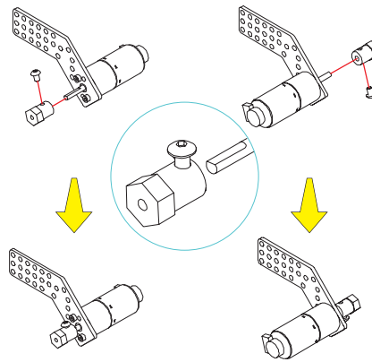
Step 2: install the right and left coupling
