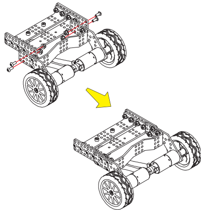
Step 8: attach the middle bracket to the front bracket
