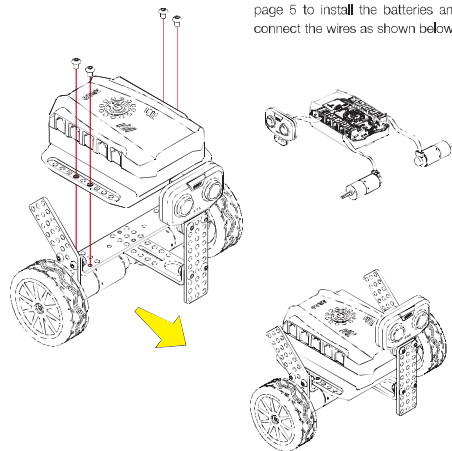
Step 8: install the main control box
