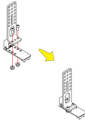
Step 9: install the tracking sensor
