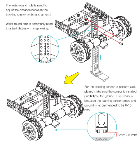
Step 10: install the tracking sensor assembly
