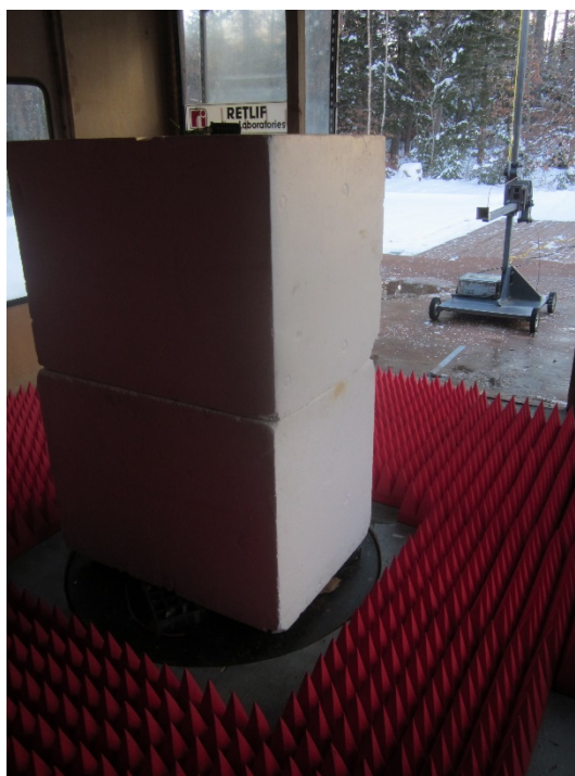
Vertical Antenna Polarization, 18 GHz to 25 GHz, Horn
