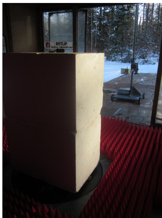
Vertical Antenna Polarization, 1 GHz to 18 GHz, Double Ridged Guide
