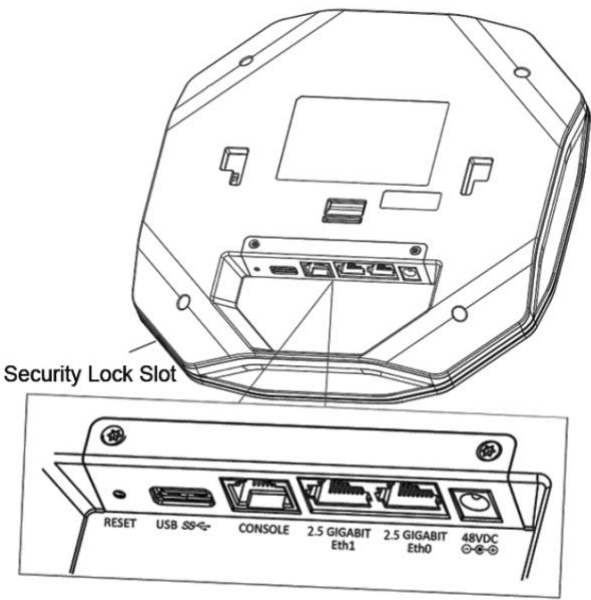
Figure 3: AP431 Back View
