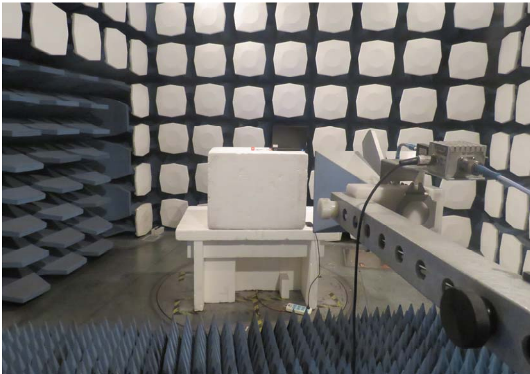
Above 1GHz
