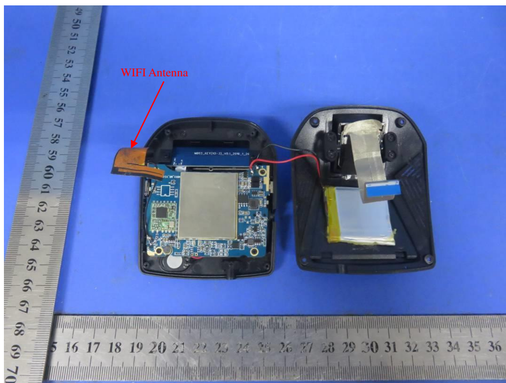
Fig.1 A305_internal_overview
