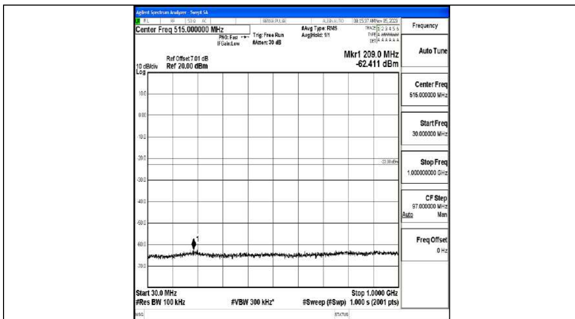
Band2_1.4MHz_16QAM_18607_1RB#0_30~1000_30~1000
