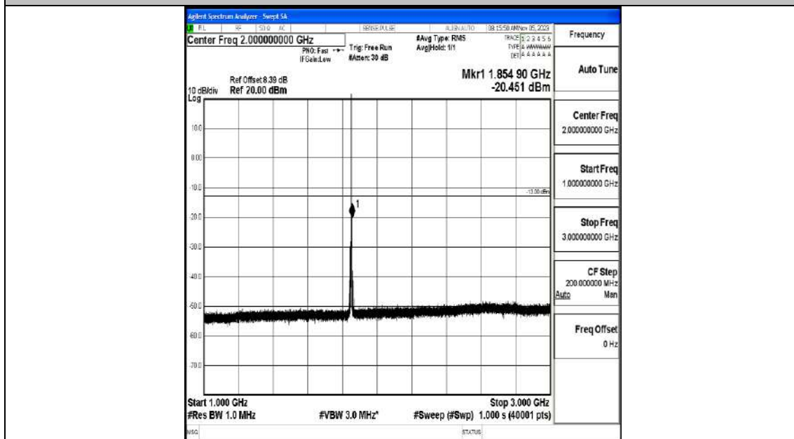
Band2_1.4MHz_16QAM_18607_1RB#0_1000~3000_1000~3000
