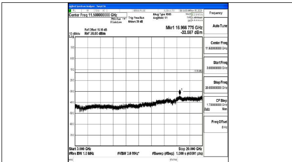
Band2_1.4MHz_16QAM_18607_1RB#0_3000~20000_3000~20000
