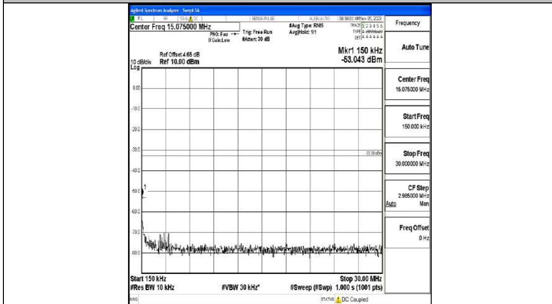
Band2_15MHz_16QAM_18675_1RB#0_0.15~30_0.15~30
