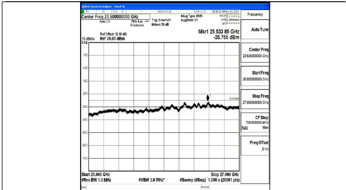
Band41_20MHz_QPSK_39750_1RB#0_20000~27000_20000~27000
