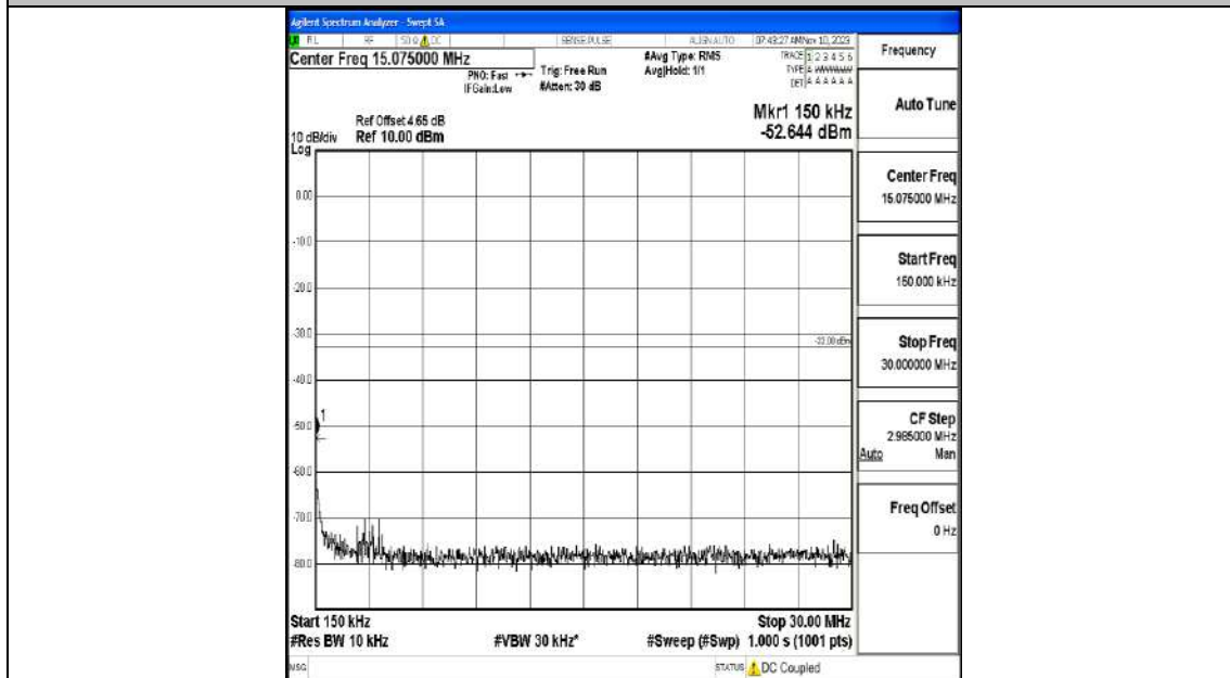
Band66_15MHz_16QAM_132047_1RB#0_0.15~30_0.15~30
