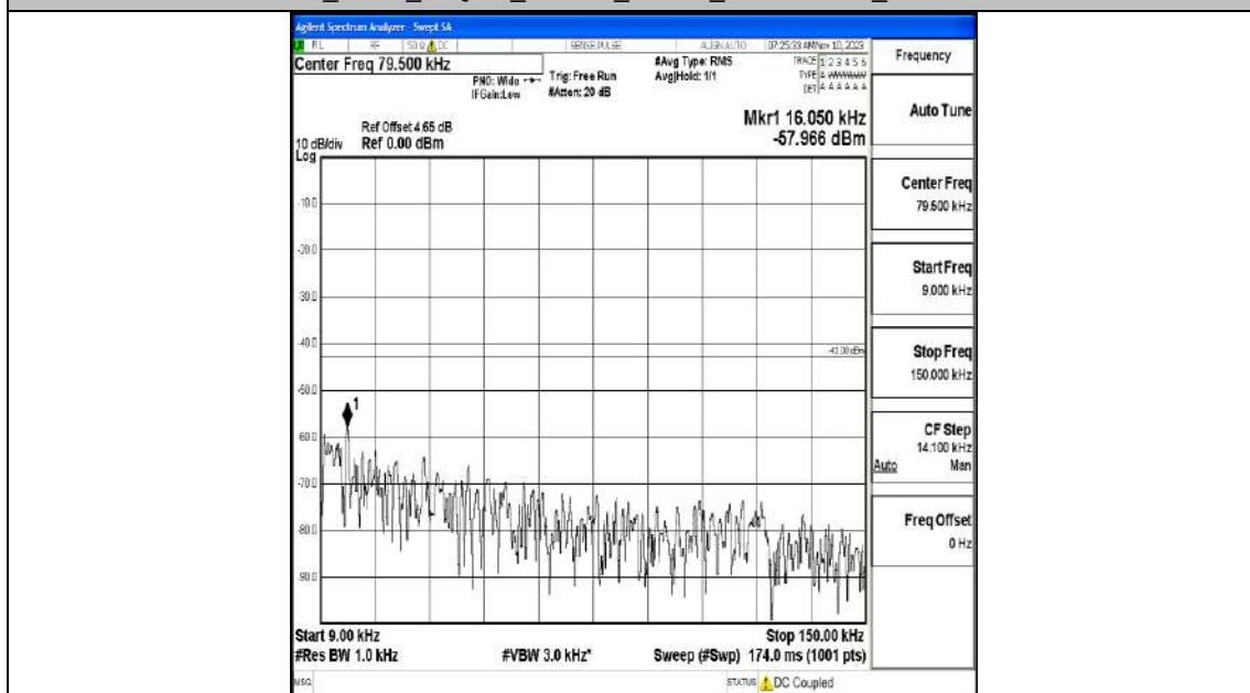
Band66 10MHz QPSK 132022 1RB#0 0.009~0.15 0.009~0.15
