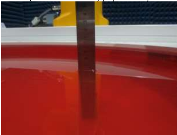
Fig. 9.3 Photo of Liquid Height for Body SAR of Twin Phantom (2000MHz~2600MHz) (depth>15cm)
