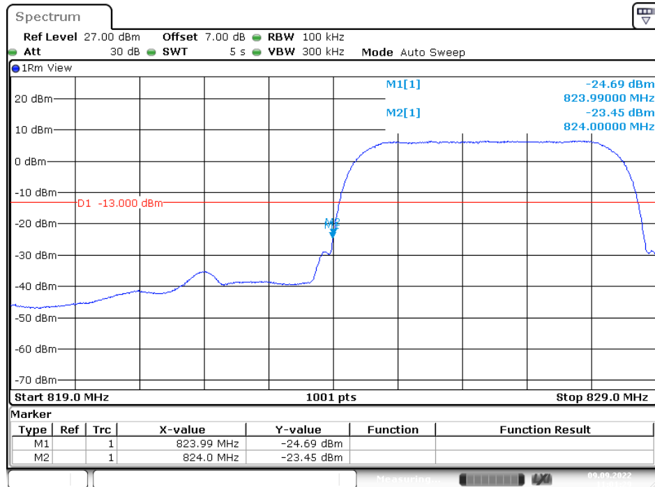
Left Band Edge for RMC (BPSK) Mode
