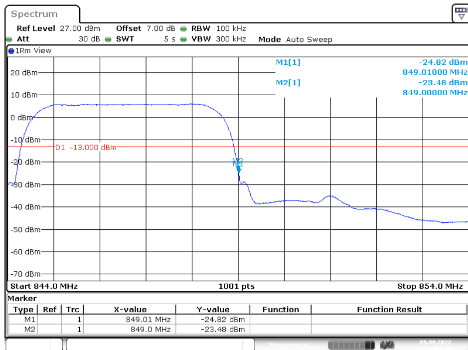
Right Band Edge for RMC (BPSK) Mode
