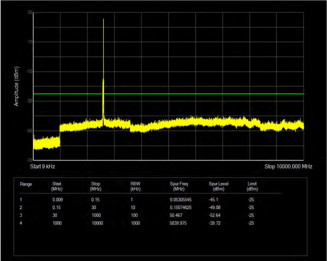
Band41(2555-2655) QPSK BW=15MHz Channel=40740 RB Size=1 Position=#Max
