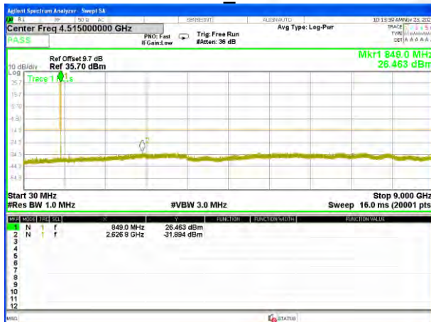
GSM850_High
