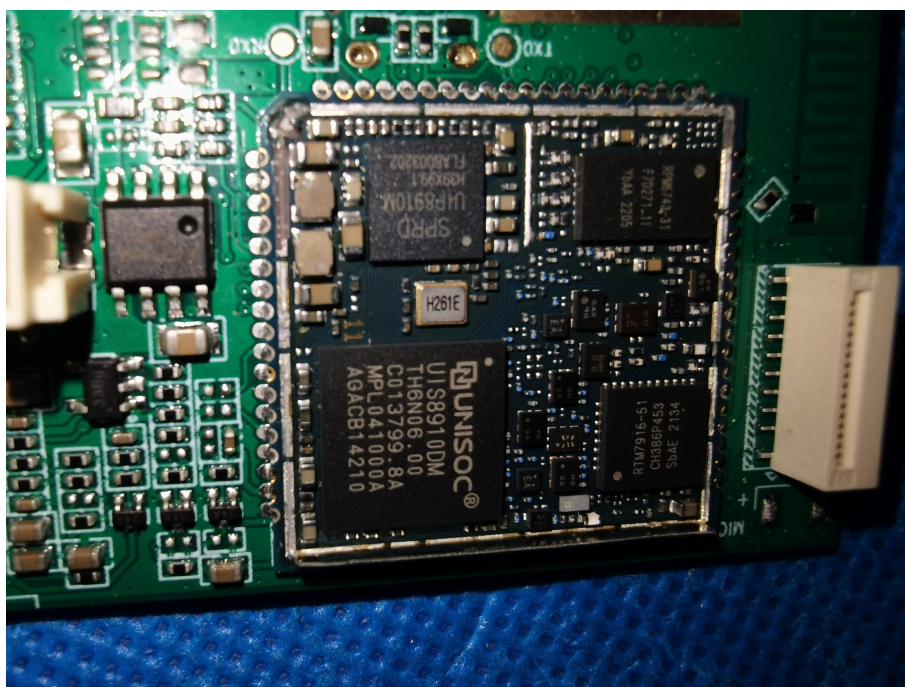
OPEN VIEW OF EUT(FIGURE 6)
