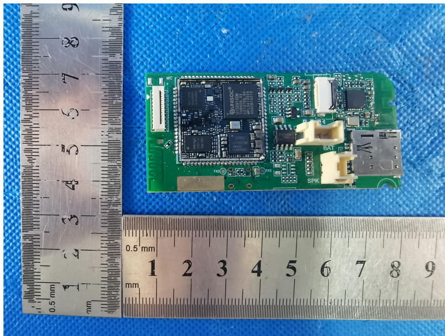
OPEN VIEW OF EUT(Figure 4)
