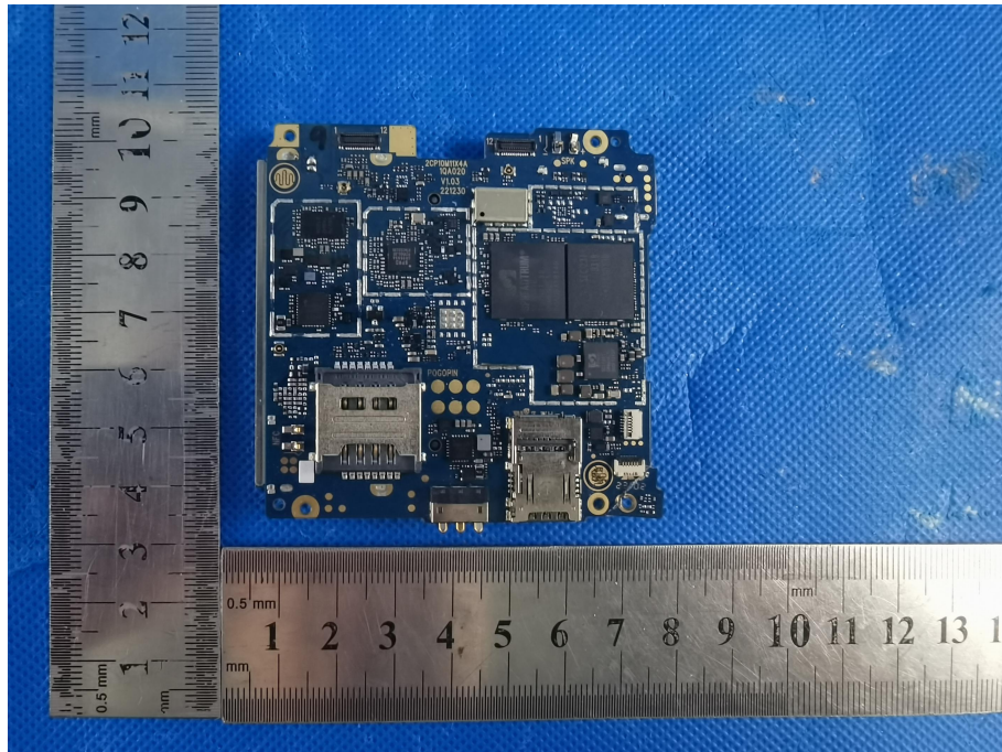
INTERNAL VIEW OF EUT(FIGURE 6)
