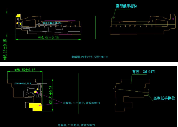
Antenna size
