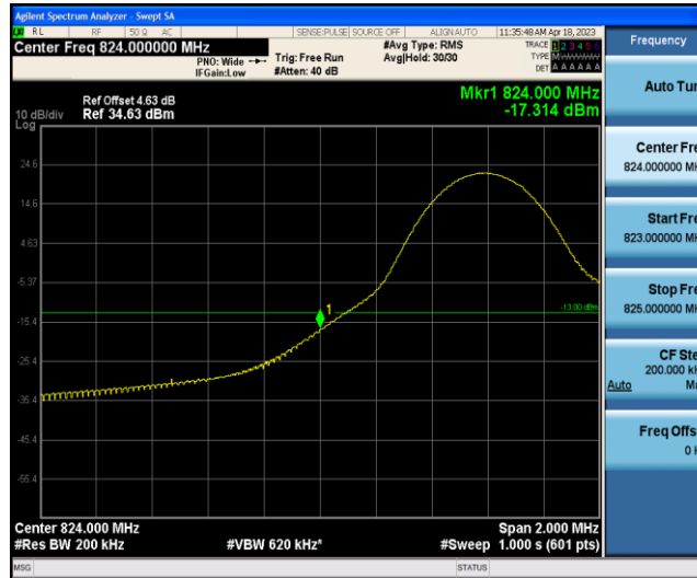
Band26-10MHz-QPSK-26840-1RB#49
