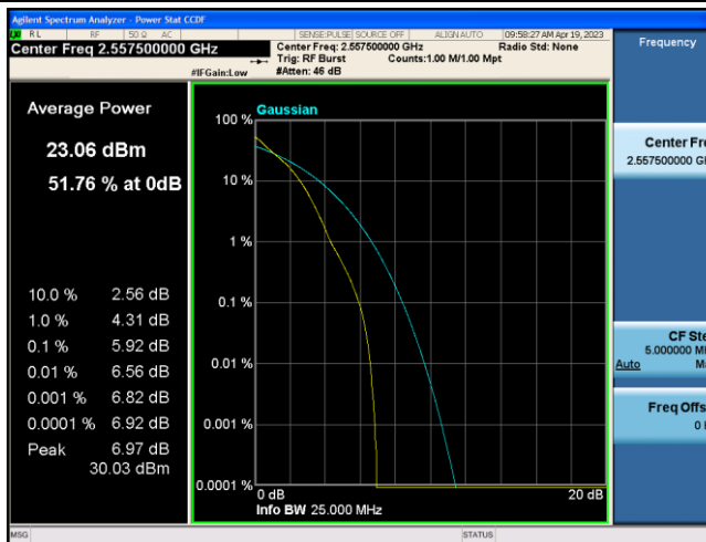
Band41-5MHz-16QAM-40265-25RB#0
