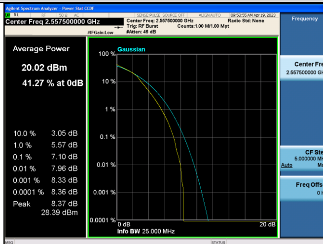
Band41-5MHz-16QAM-40265-25RB#0
