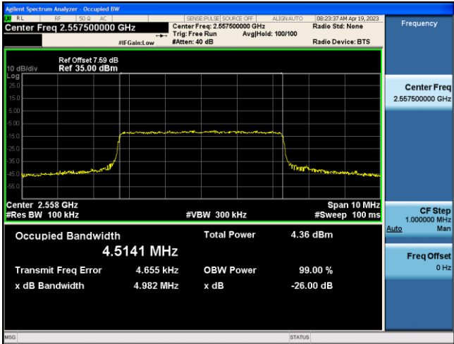
Band41-5MHz-QPSK-40265-25RB#0
