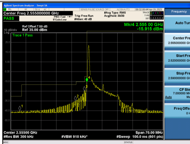
Band41-15MHz-QPSK-40315-1RB#74
