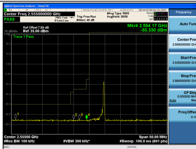
Band41-5MHz-16QAM-40265-25RB#0
