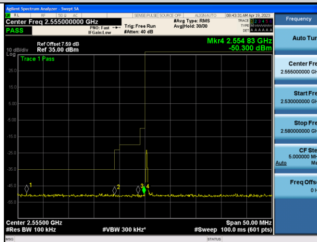
Band41-5MHz-16QAM-40265-1RB#24
