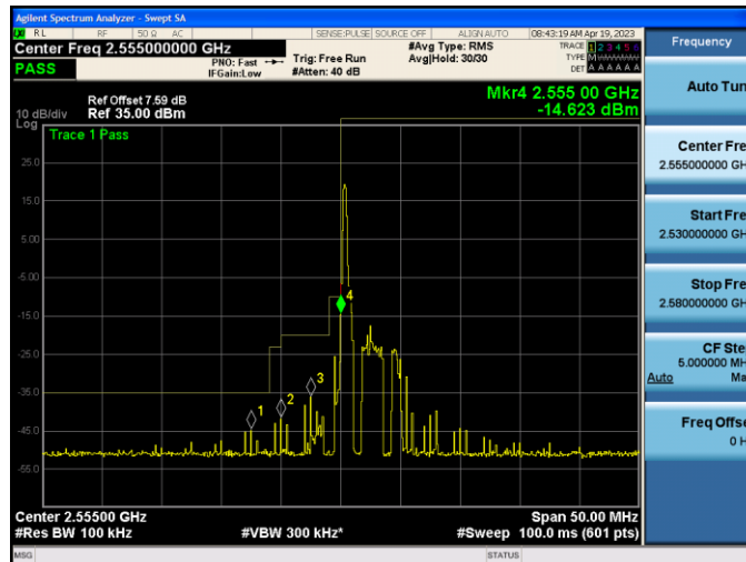
Band41-5MHz-QPSK-40265-1RB#24
