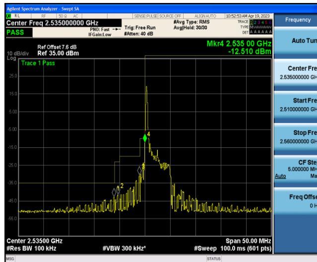
Band41-5MHz-16QAM-40065-1RB#24
