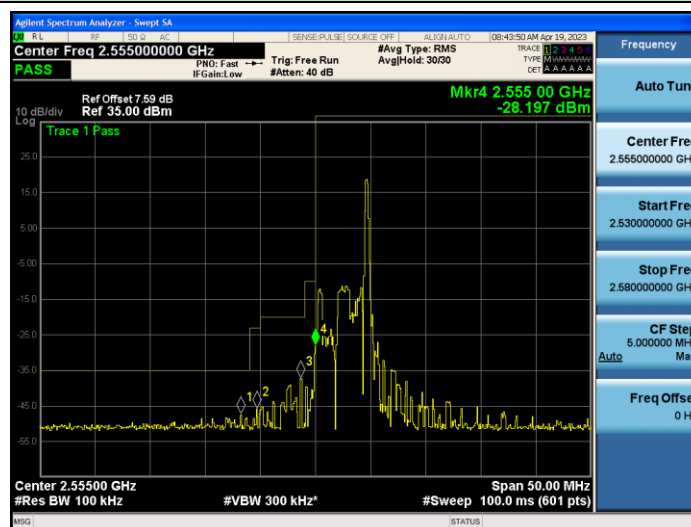
Band41-5MHz-QPSK-40265-25RB#0
