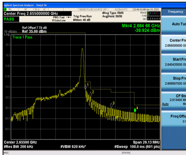
Band41-10MHz-QPSK-41190-50RB#0
