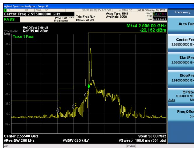
Band41-10MHz-16QAM-40290-1RB#49
