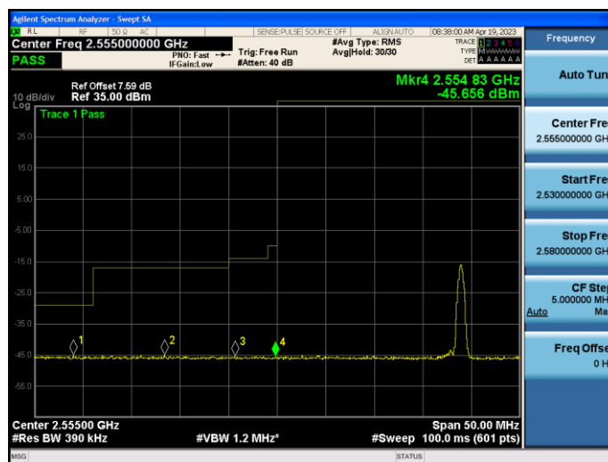
Band41-20MHz-16QAM-40340-100RB#0
