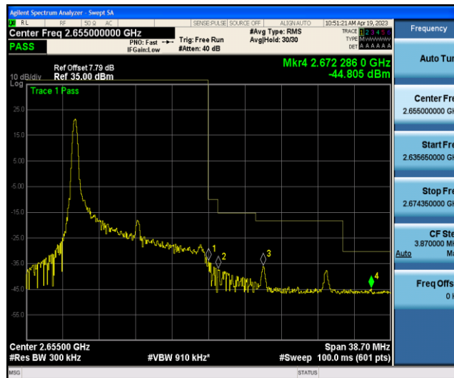
Band41-15MHz-16QAM-41165-1RB#74
