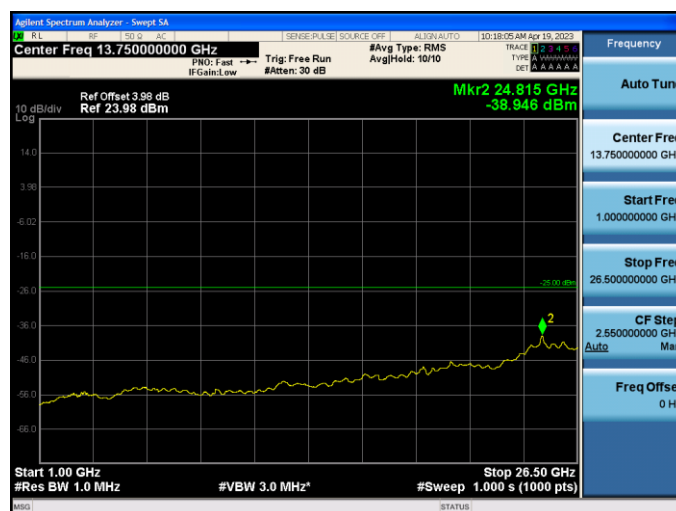
Band41-5MHz-16QAM-40265-1RB#0-Range2:1000~26500MHz
