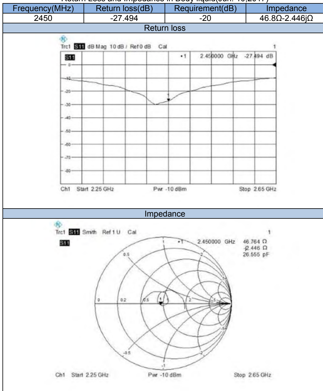
Return Loss and Impedance in Body liquid(Jun. 10,2017)
