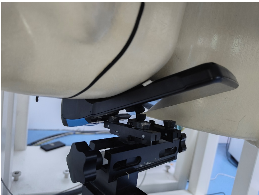
Handheld Back (Wi-Fi & BT Ant) Setup Photo
