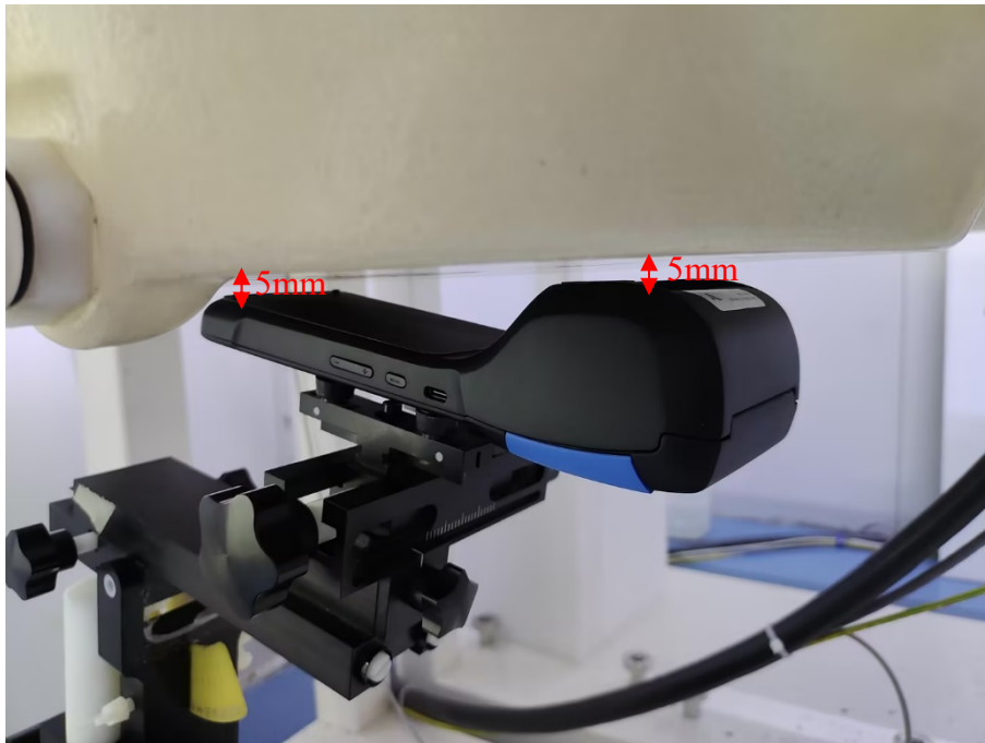
Handheld Front Setup Photo
