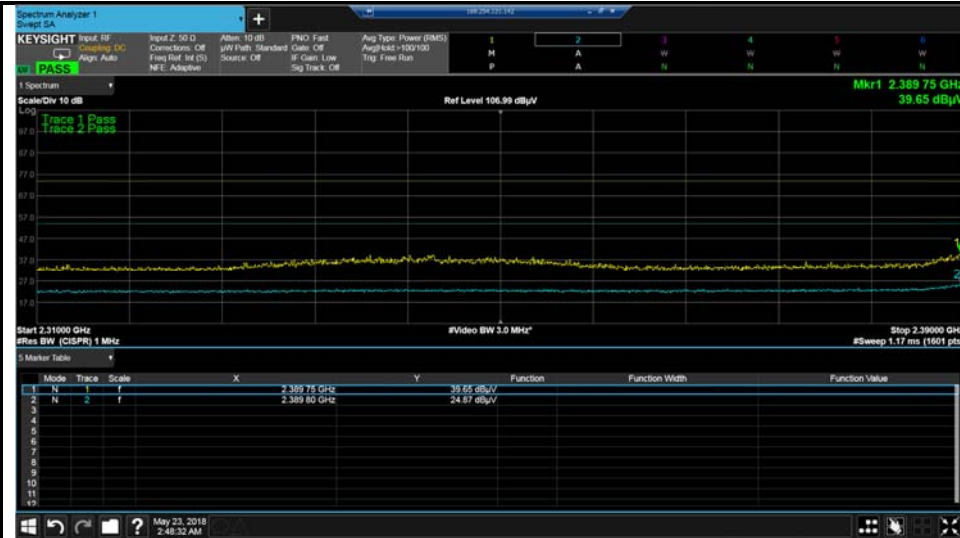
2.4GHz-11N20-2412 MHz
