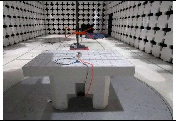
Radiated Emissions (<1GHz) – Rear View
