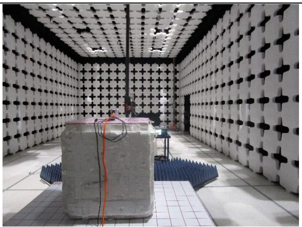
Radiated Emissions (Above 1G) – Rear View
