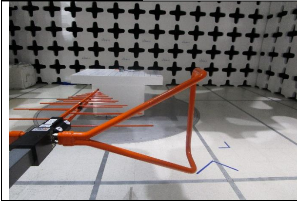
Radiated Emissions (<1GHz) – Front View
