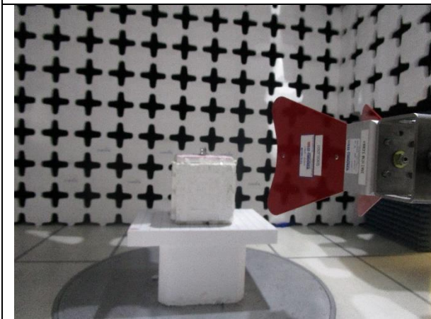
Radiated Emissions (Above 1G) – Front View
