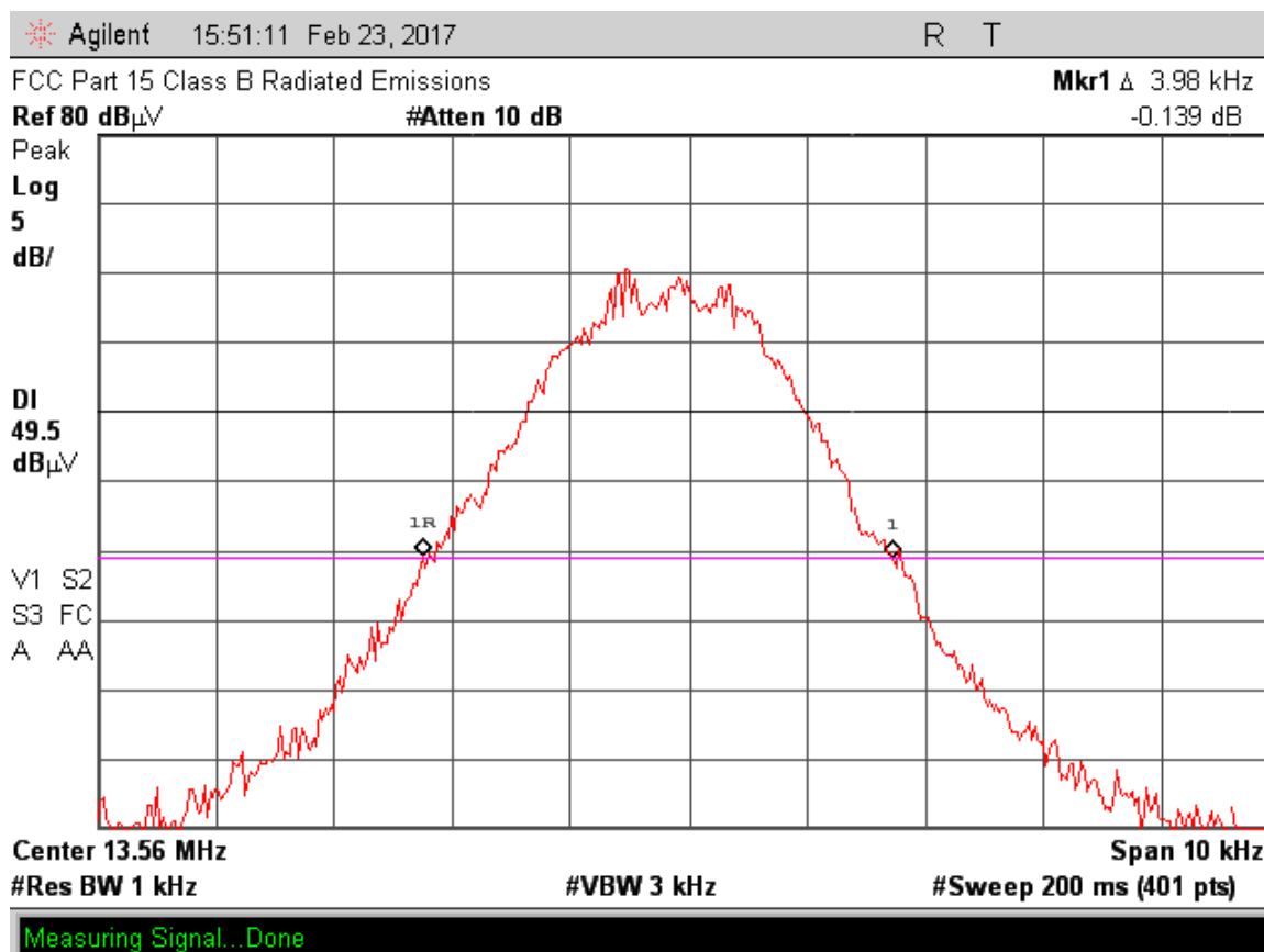
Figure 2.2.8-1 – Bandwidth Plot
