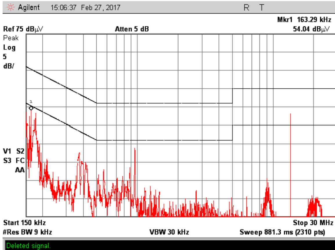
Figure 2.5.11-1 – Conducted Emissions Plot
