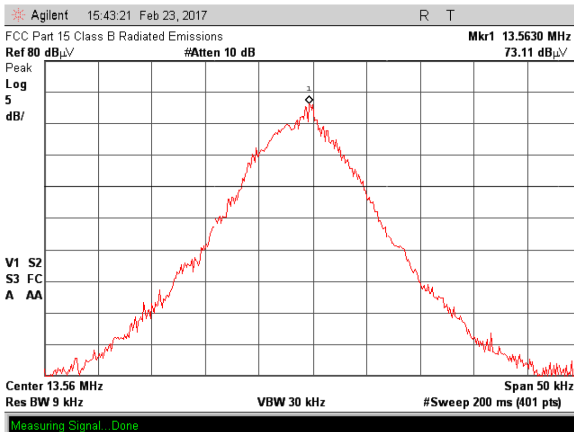
Figure 2.3.11-1 – Field Strength Plot of the Fundamental Emission
