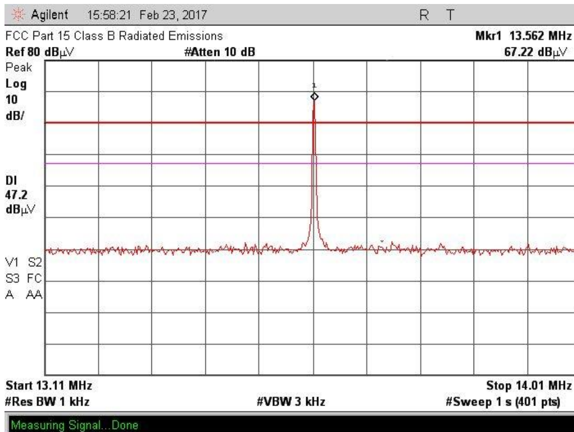
Figure 2.3.11-2 – Emissions within the 13.1 MHz to 14.01 MHz Band
