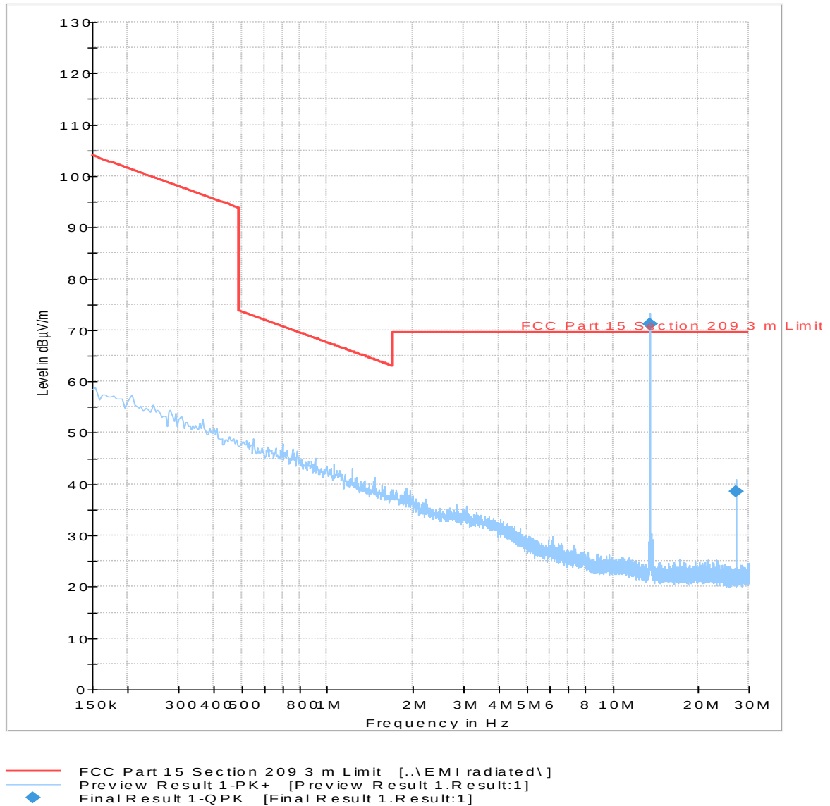
Figure 2.4.10-1 – Radiated Emissions Data 150 kHz – 30 MHz
