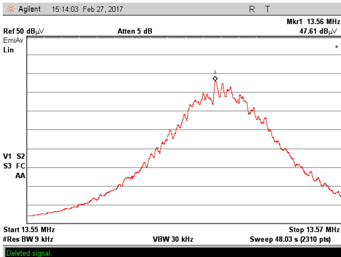
Figure 2.5.11-2 – Conducted Emissions Plot – Average Detector
