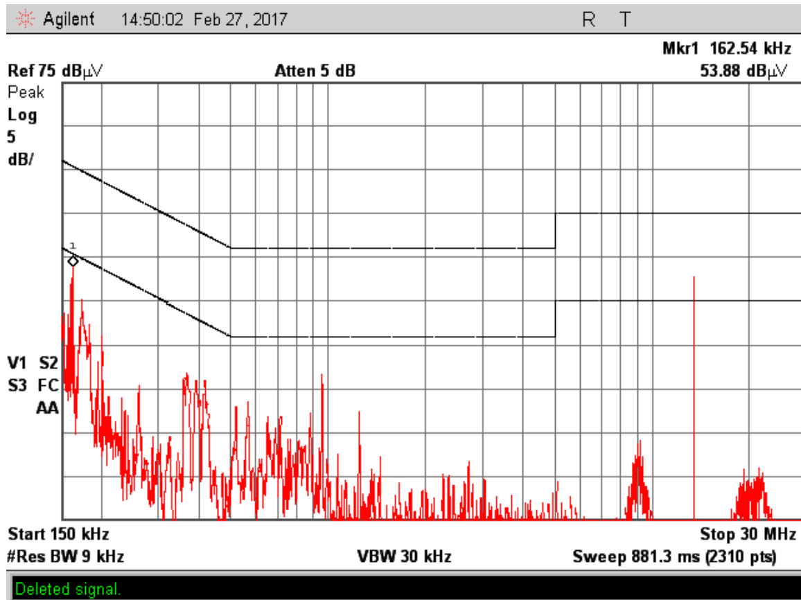
Figure 2.5.10-1 – Conducted Emissions Plot
