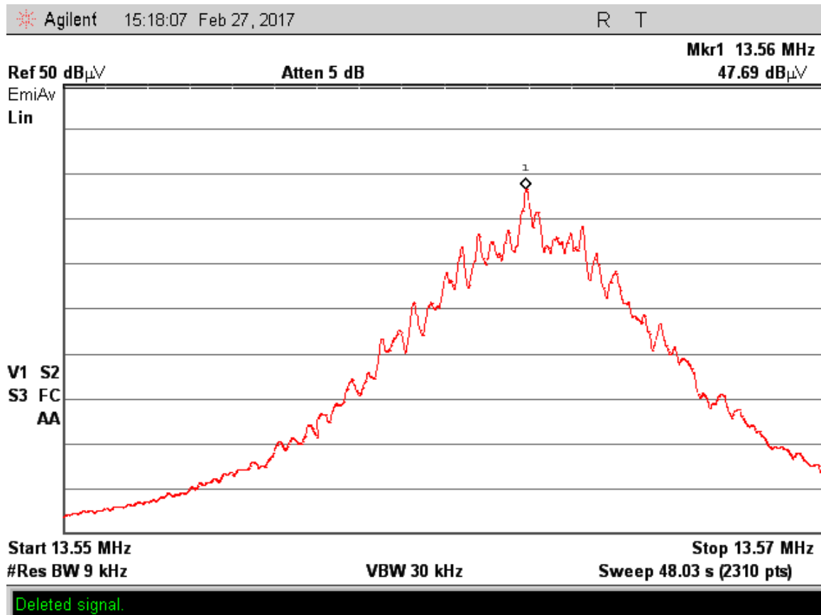
Figure 2.5.10-2 – Conducted Emissions Plot – Average Detector
