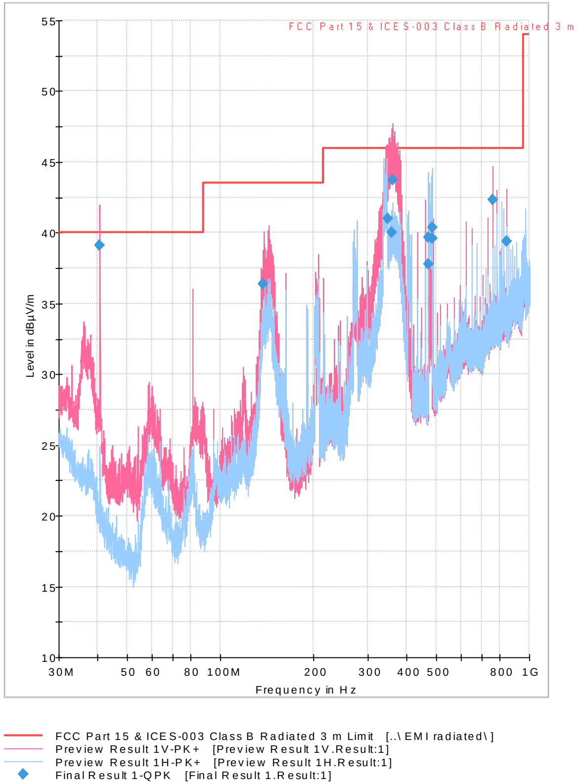
Figure 2.4.11-1 – Radiated Emissions 30 MHz to 1 GHz Plot
