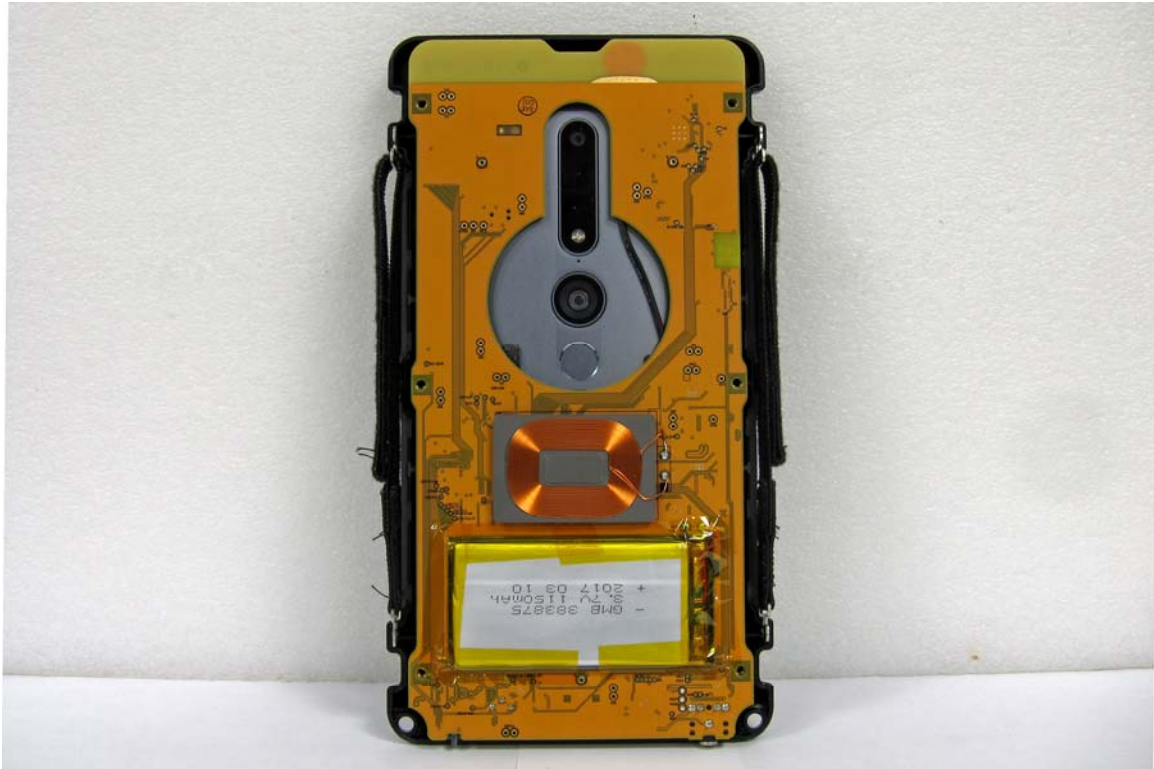
Docent Rear Cover Removed
